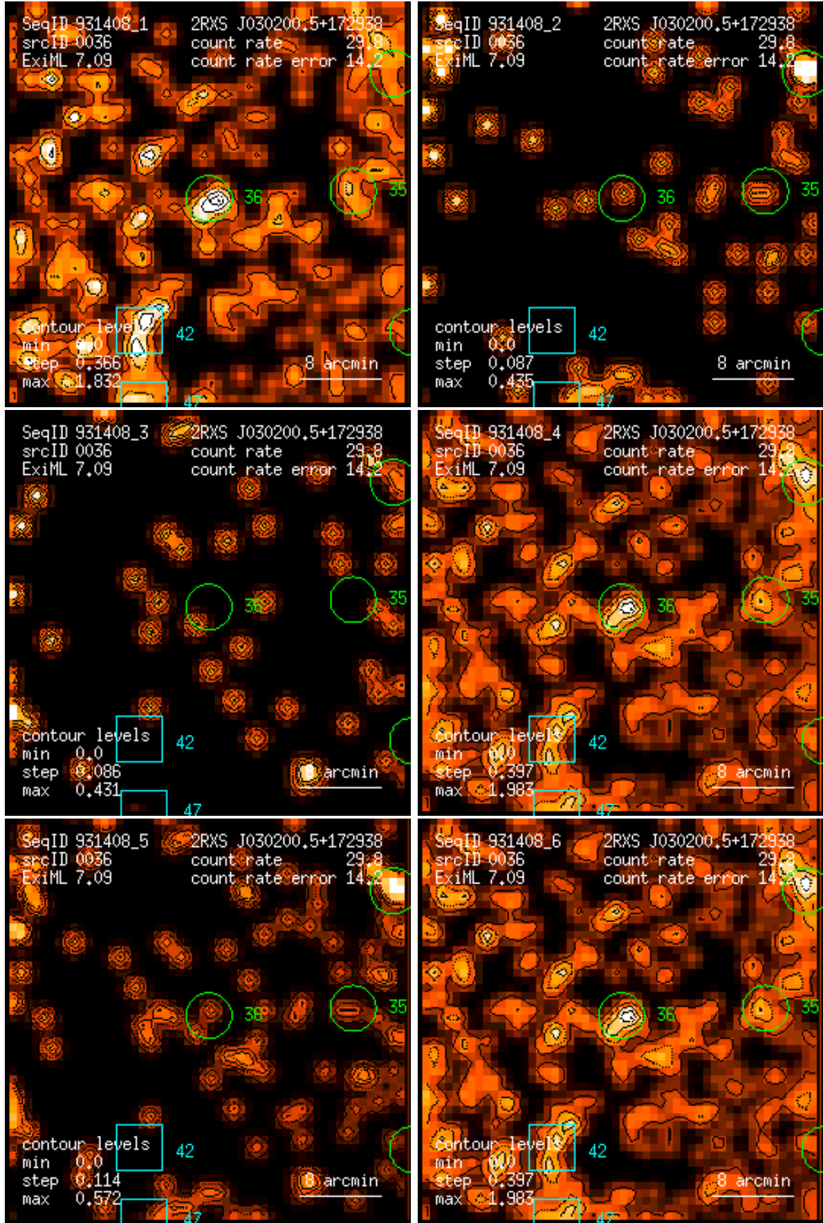
Figure 36: RASS 931408: detection 0036: band rate images, Gaussian filter: (1) PSPC channels 11 – 41, (2) 52 – 90, (3) 91 – 201, (4) 11 – 235, (5) 52 – 201, (6) 11 – 201. Broad band rates in counts/ks. Band rate contour levels in counts/ks/arcmin 2 .
