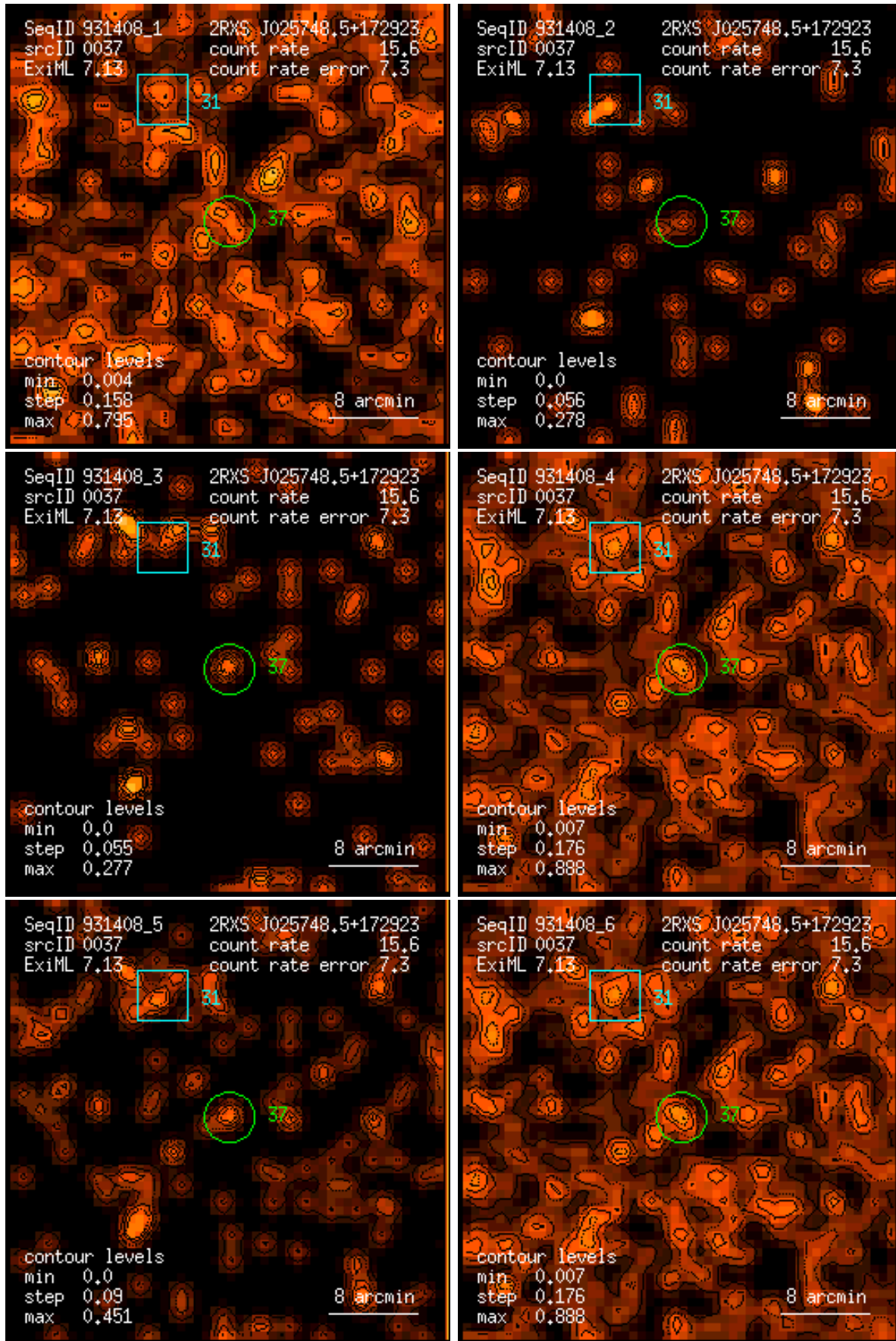
Figure 37: RASS 931408: detection 0037: band rate images, Gaussian filter: (1) PSPC channels 11 – 41, (2) 52 – 90, (3) 91 – 201, (4) 11 – 235, (5) 52 – 201, (6) 11 – 201. Broad band rates in counts/ks. Band rate contour levels in counts/ks/arcmin 2 .
