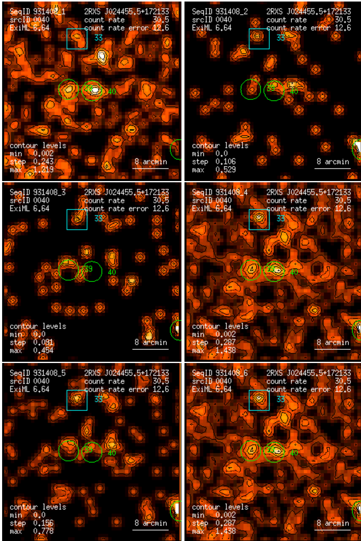
Figure 40: RASS 931408: detection 0040: band rate images, Gaussian filter: (1) PSPC channels 11 – 41, (2) 52 – 90, (3) 91 – 201, (4) 11 – 235, (5) 52 – 201, (6) 11 – 201. Broad band rates in counts/ks. Band rate contour levels in counts/ks/arcmin 2 .
