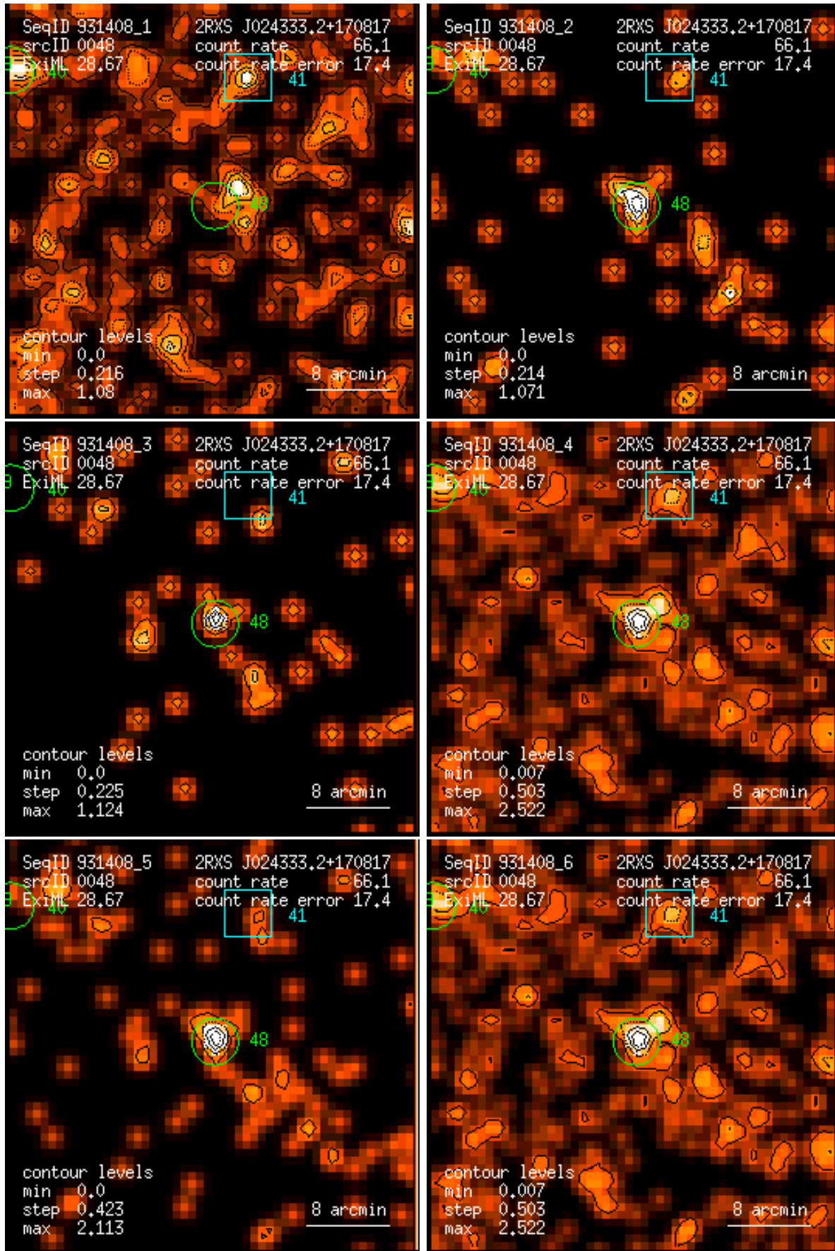
Figure 48: RASS 931408: detection 0048: band rate images, Gaussian filter: (1) PSPC channels 11 – 41, (2) 52 – 90, (3) 91 – 201, (4) 11 – 235, (5) 52 – 201, (6) 11 – 201. Broad band rates in counts/ks. Band rate contour levels in counts/ks/arcmin 2 .
