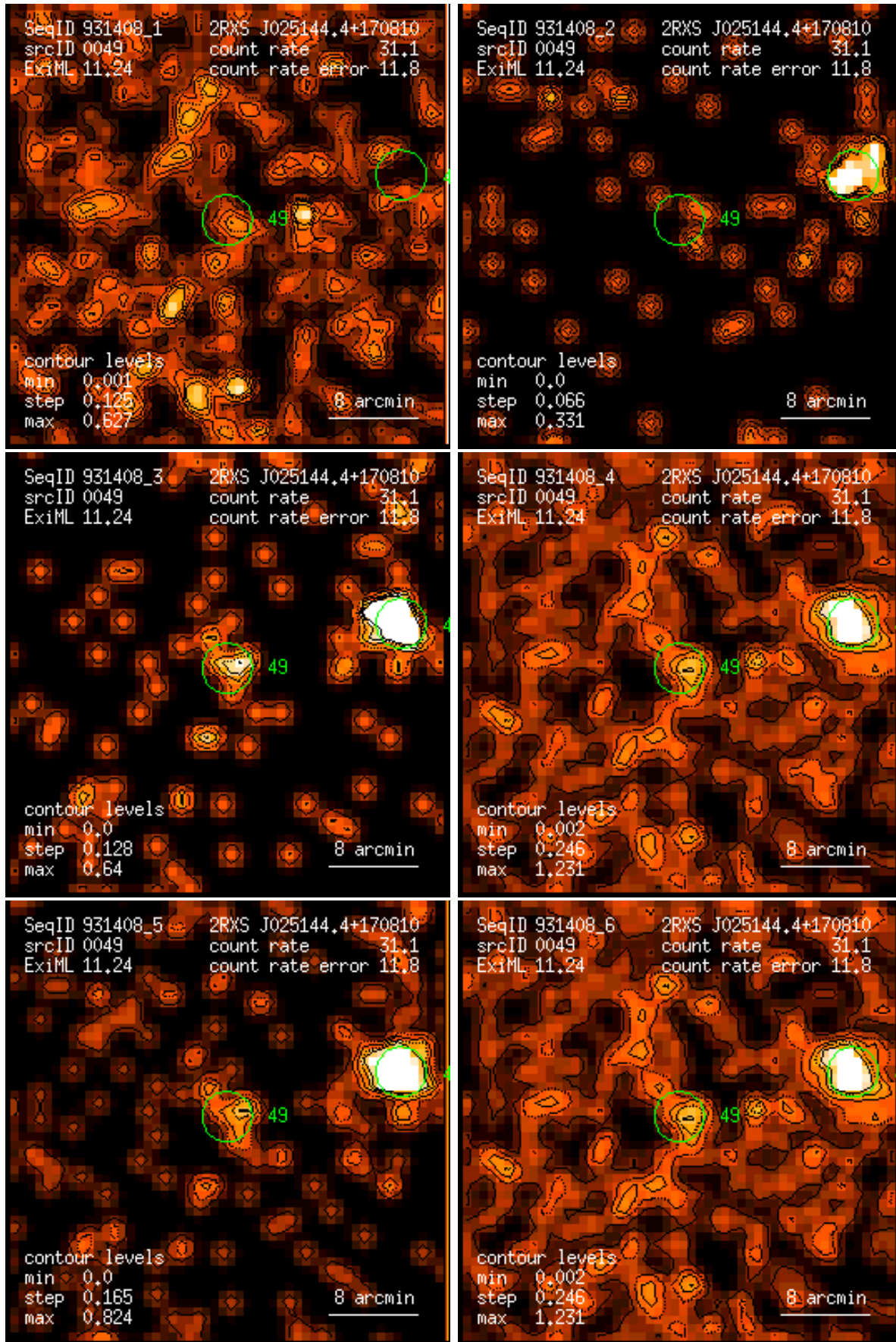
Figure 49: RASS 931408: detection 0049: band rate images, Gaussian filter: (1) PSPC channels 11 – 41, (2) 52 – 90, (3) 91 – 201, (4) 11 – 235, (5) 52 – 201, (6) 11 – 201. Broad band rates in counts/ks. Band rate contour levels in counts/ks/arcmin 2 .
