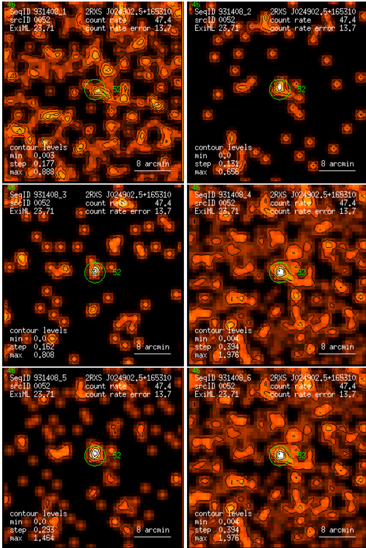
Figure 52: RASS 931408: detection 0052: band rate images, Gaussian filter: (1) PSPC channels 11 – 41, (2) 52 – 90, (3) 91 – 201, (4) 11 – 235, (5) 52 – 201, (6) 11 – 201. Broad band rates in counts/ks. Band rate contour levels in counts/ks/arcmin 2 .
