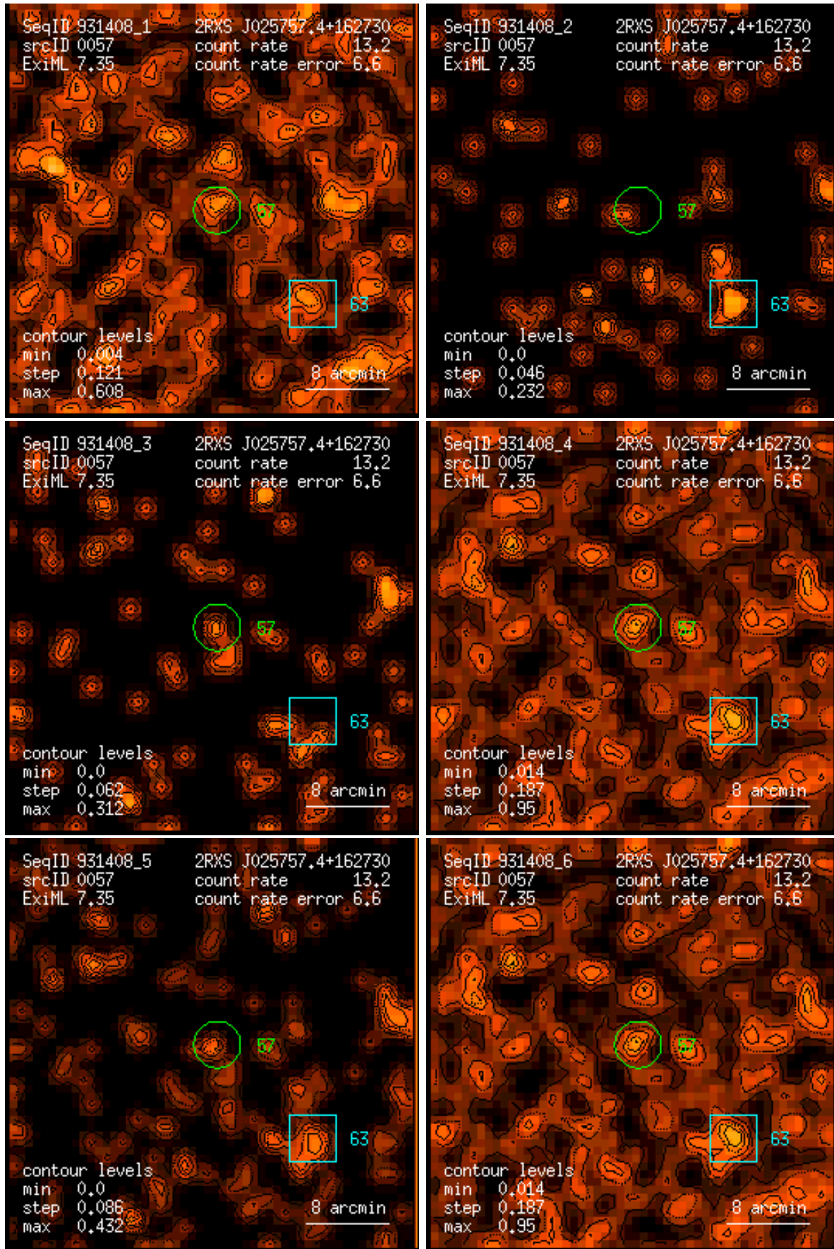
Figure 57: RASS 931408: detection 0057: band rate images, Gaussian filter: (1) PSPC channels 11 – 41, (2) 52 – 90, (3) 91 – 201, (4) 11 – 235, (5) 52 – 201, (6) 11 – 201. Broad band rates in counts/ks. Band rate contour levels in counts/ks/arcmin 2 .
