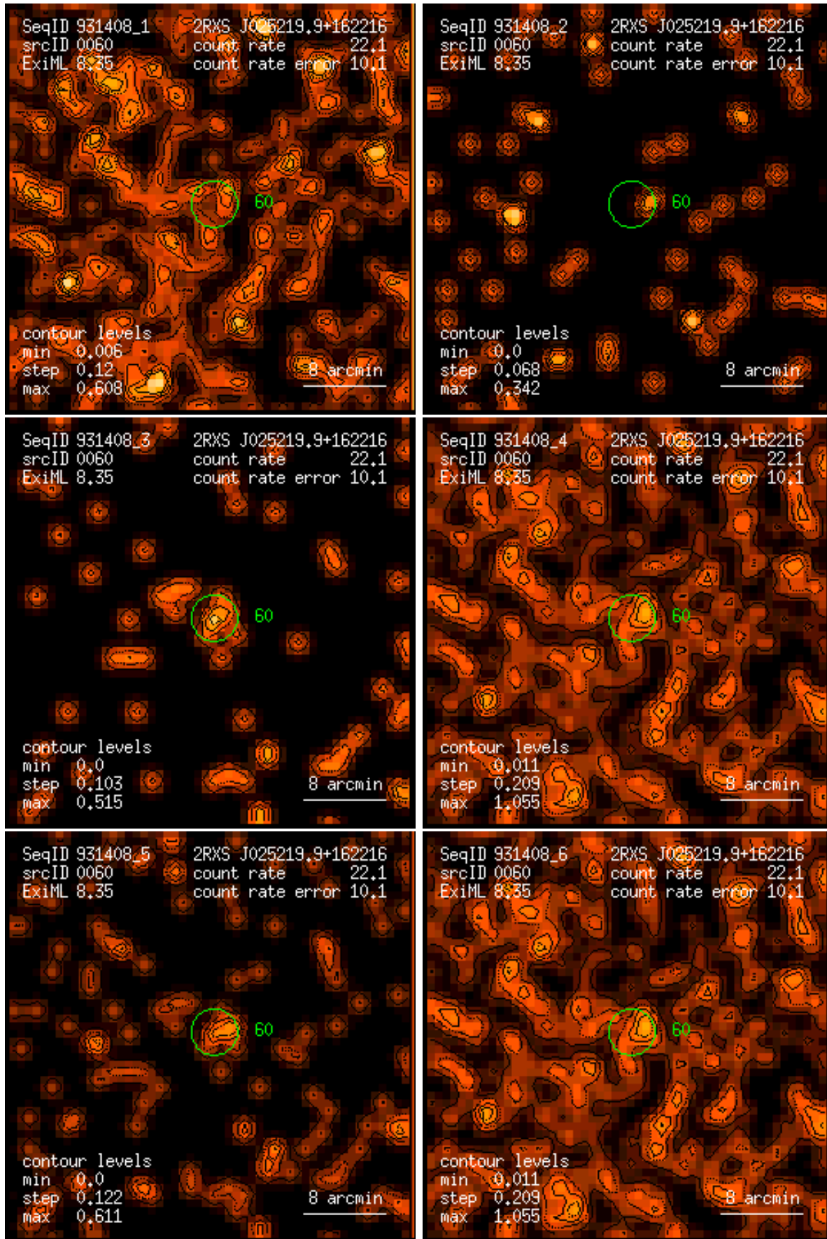
Figure 60: RASS 931408: detection 0060: band rate images, Gaussian filter: (1) PSPC channels 11 – 41, (2) 52 – 90, (3) 91 – 201, (4) 11 – 235, (5) 52 – 201, (6) 11 – 201. Broad band rates in counts/ks. Band rate contour levels in counts/ks/arcmin 2 .
