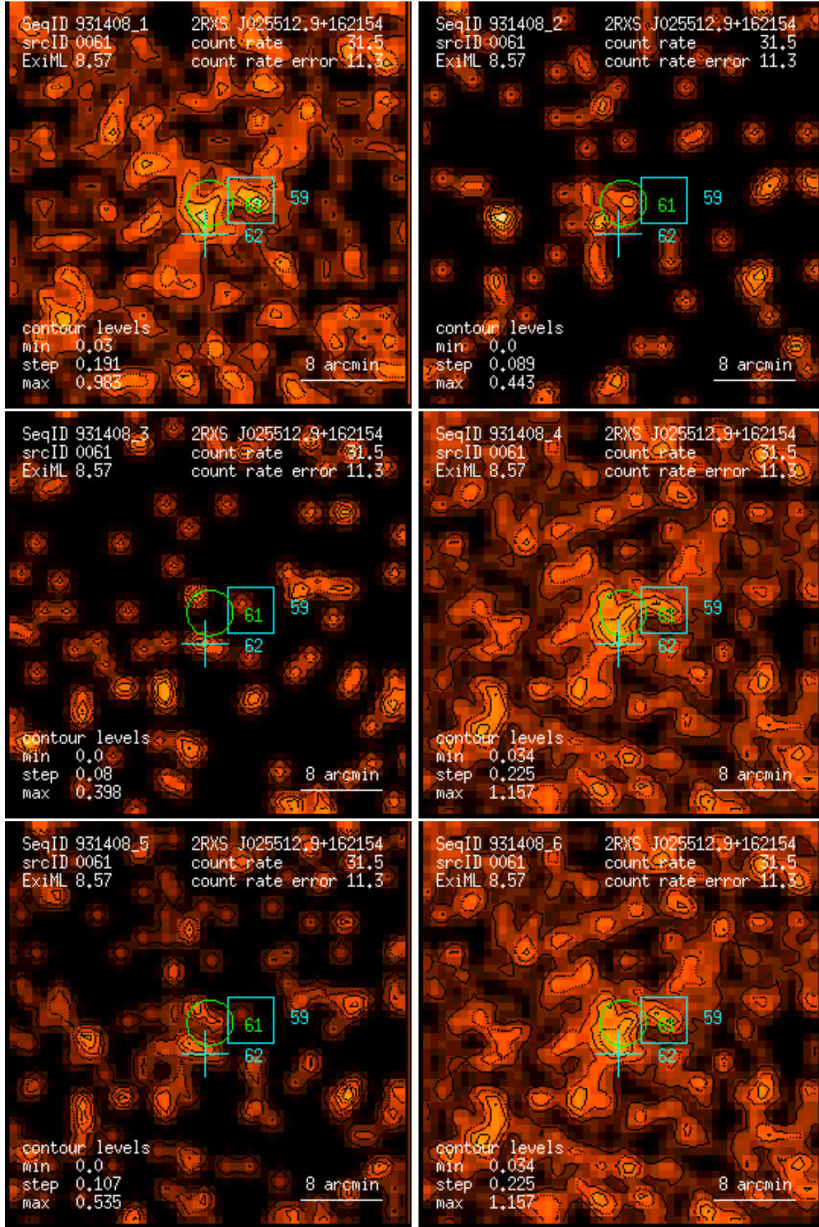
Figure 61: RASS 931408: detection 0061: band rate images, Gaussian filter: (1) PSPC channels 11 – 41, (2) 52 – 90, (3) 91 – 201, (4) 11 – 235, (5) 52 – 201, (6) 11 – 201. Broad band rates in counts/ks. Band rate contour levels in counts/ks/arcmin 2 .
