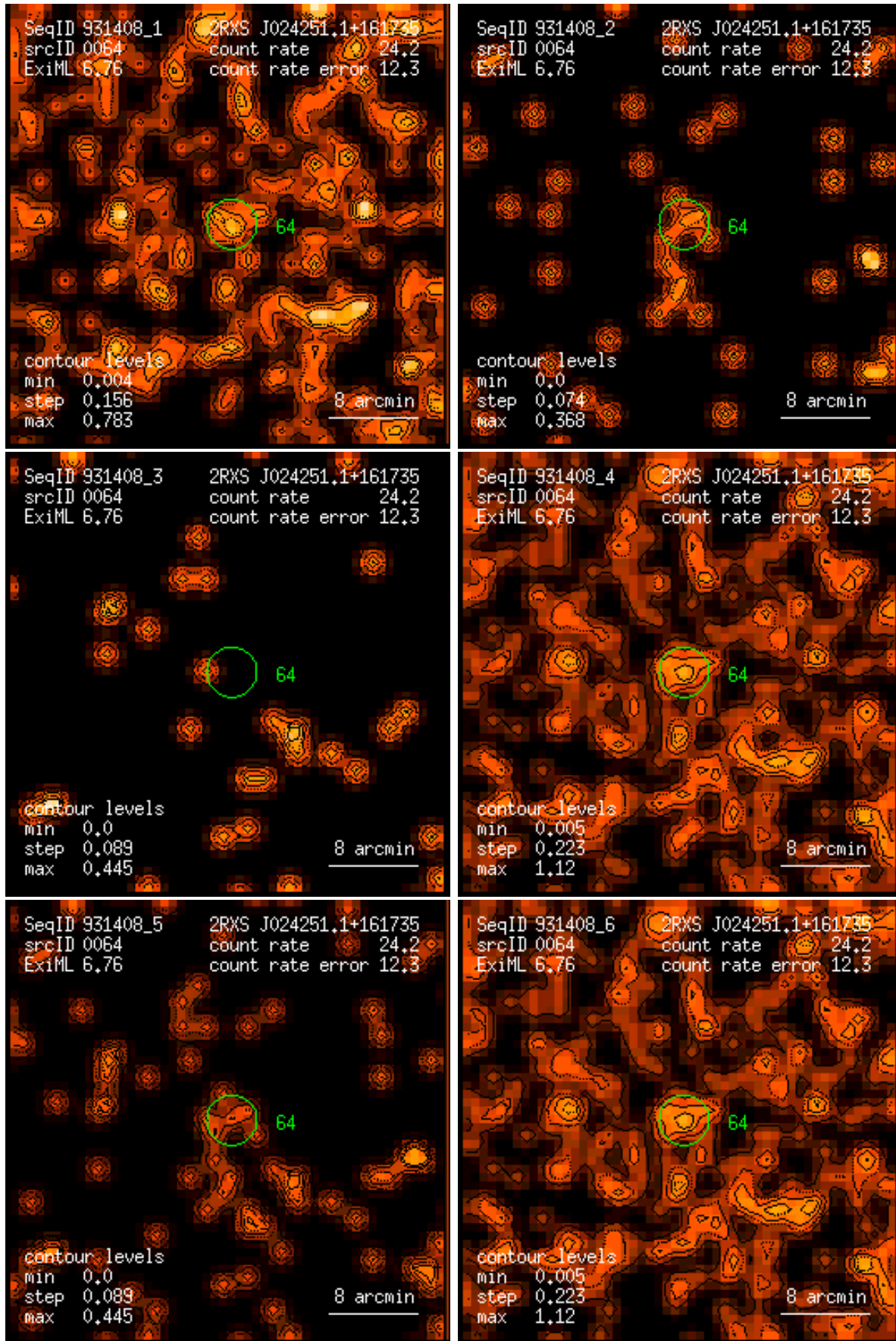
Figure 64: RASS 931408: detection 0064: band rate images, Gaussian filter: (1) PSPC channels 11 – 41, (2) 52 – 90, (3) 91 – 201, (4) 11 – 235, (5) 52 – 201, (6) 11 – 201. Broad band rates in counts/ks. Band rate contour levels in counts/ks/arcmin 2 .
