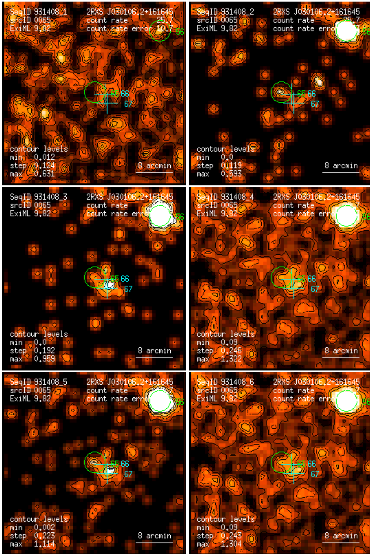
Figure 65: RASS 931408: detection 0065: band rate images, Gaussian filter: (1) PSPC channels 11 – 41, (2) 52 – 90, (3) 91 – 201, (4) 11 – 235, (5) 52 – 201, (6) 11 – 201. Broad band rates in counts/ks. Band rate contour levels in counts/ks/arcmin 2 .
