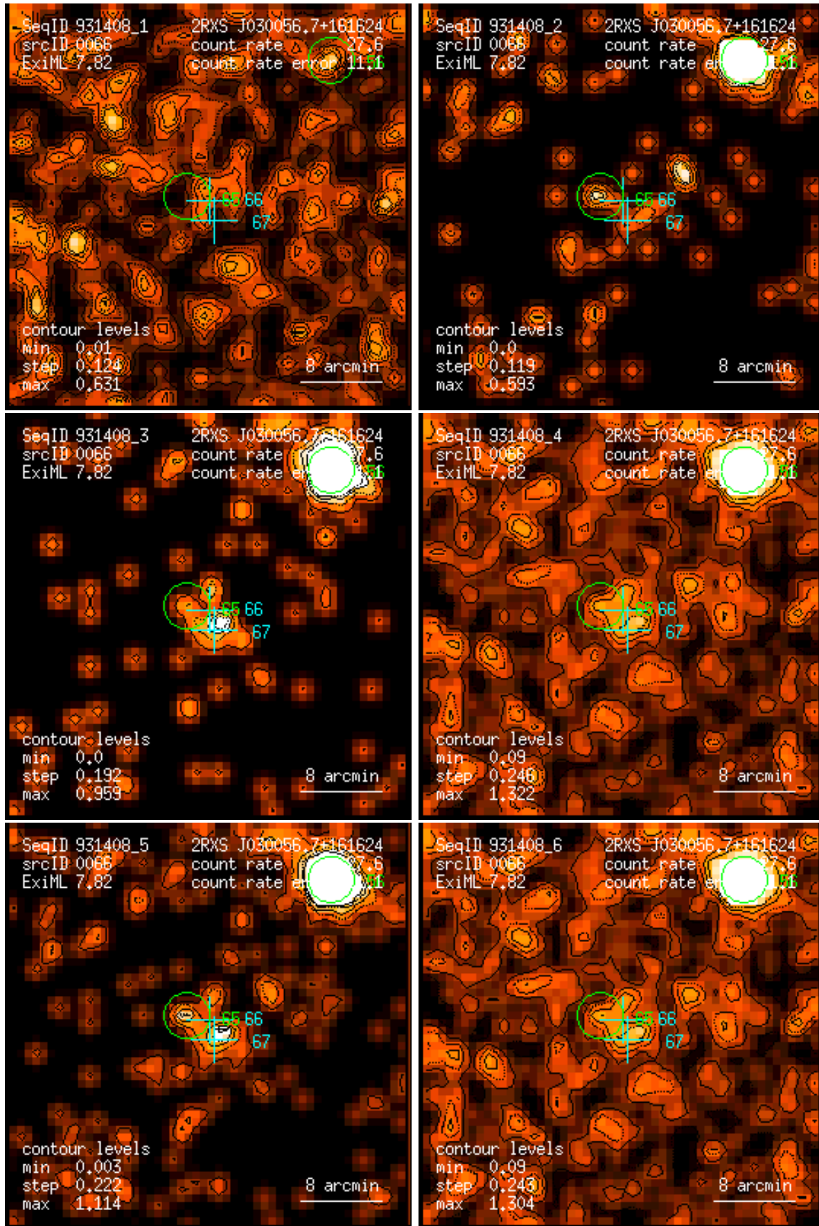
Figure 66: RASS 931408: detection 0066: band rate images, Gaussian filter: (1) PSPC channels 11 – 41, (2) 52 – 90, (3) 91 – 201, (4) 11 – 235, (5) 52 – 201, (6) 11 – 201. Broad band rates in counts/ks. Band rate contour levels in counts/ks/arcmin 2 .
