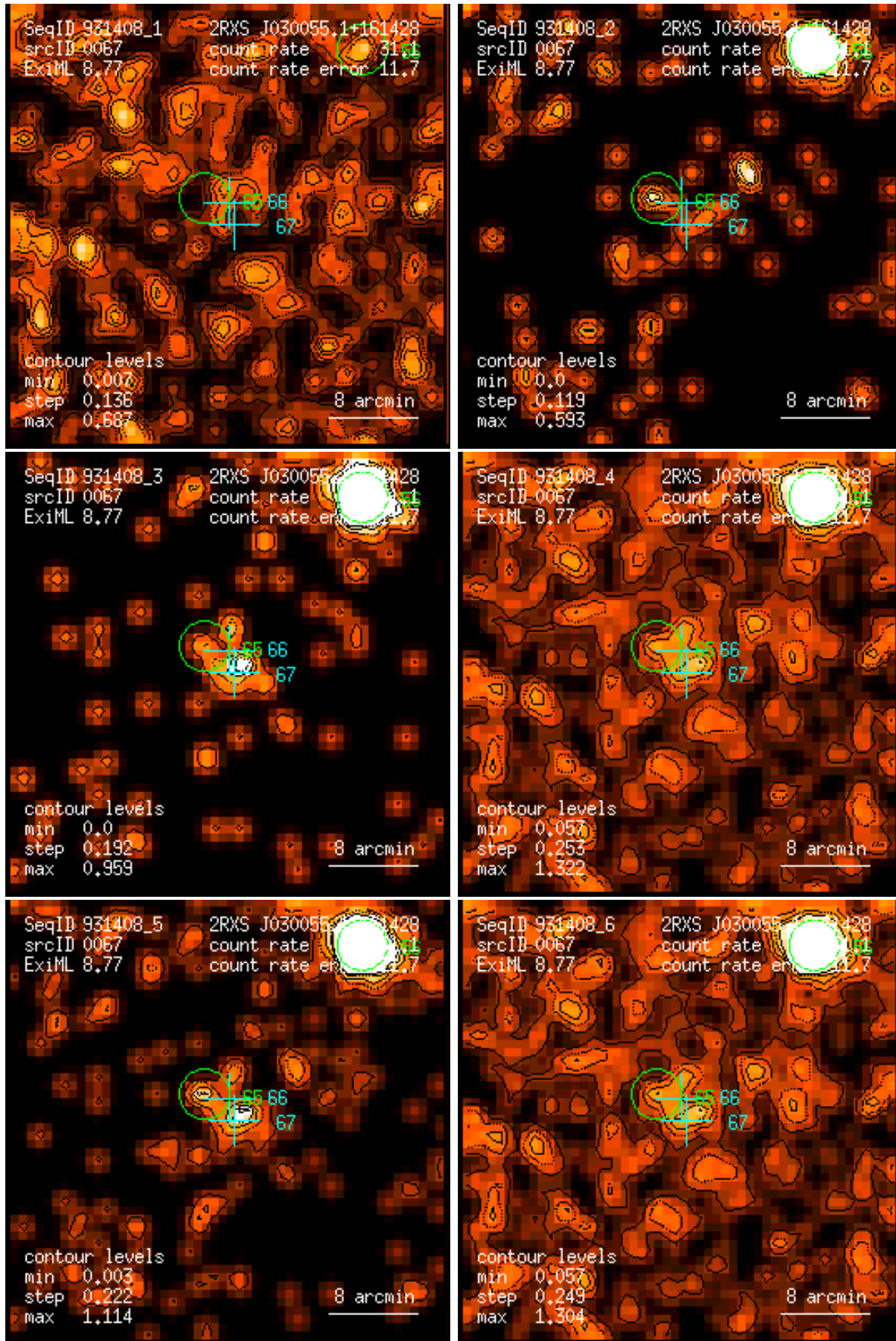
Figure 67: RASS 931408: detection 0067: band rate images, Gaussian filter: (1) PSPC channels 11 – 41, (2) 52 – 90, (3) 91 – 201, (4) 11 – 235, (5) 52 – 201, (6) 11 – 201. Broad band rates in counts/ks. Band rate contour levels in counts/ks/arcmin 2 .
