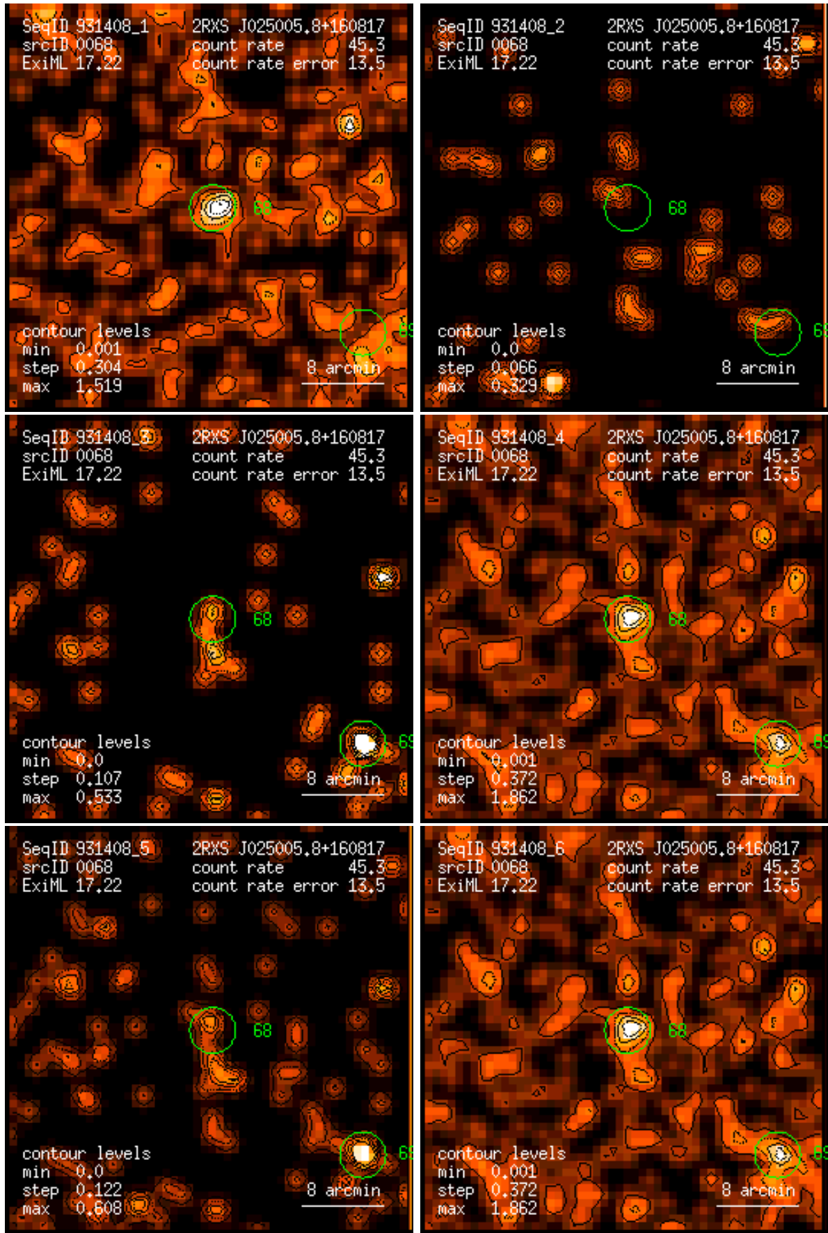
Figure 68: RASS 931408: detection 0068: band rate images, Gaussian filter: (1) PSPC channels 11 – 41, (2) 52 – 90, (3) 91 – 201, (4) 11 – 235, (5) 52 – 201, (6) 11 – 201. Broad band rates in counts/ks. Band rate contour levels in counts/ks/arcmin 2 .
