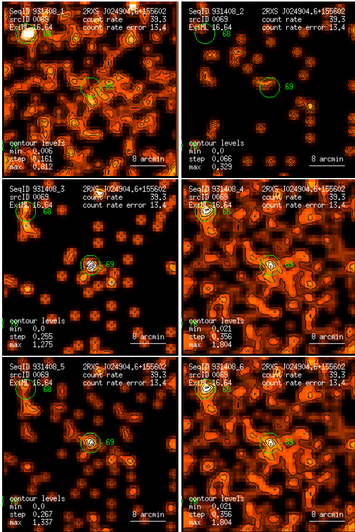
Figure 69: RASS 931408: detection 0069: band rate images, Gaussian filter: (1) PSPC channels 11 – 41, (2) 52 – 90, (3) 91 – 201, (4) 11 – 235, (5) 52 – 201, (6) 11 – 201. Broad band rates in counts/ks. Band rate contour levels in counts/ks/arcmin 2 .
