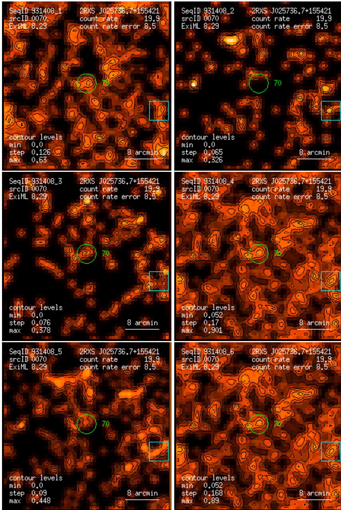
Figure 70: RASS 931408: detection 0070: band rate images, Gaussian filter: (1) PSPC channels 11 – 41, (2) 52 – 90, (3) 91 – 201, (4) 11 – 235, (5) 52 – 201, (6) 11 – 201. Broad band rates in counts/ks. Band rate contour levels in counts/ks/arcmin 2 .
