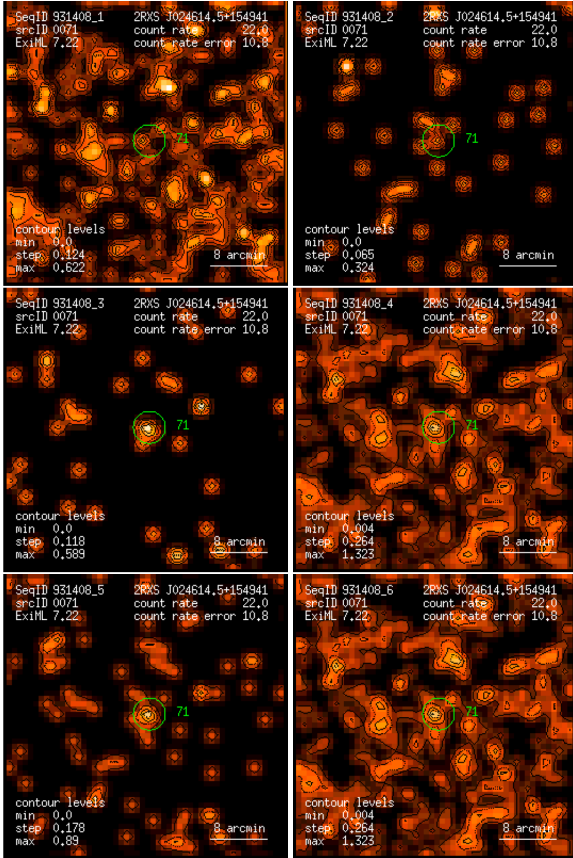
Figure 71: RASS 931408: detection 0071: band rate images, Gaussian filter: (1) PSPC channels 11 – 41, (2) 52 – 90, (3) 91 – 201, (4) 11 – 235, (5) 52 – 201, (6) 11 – 201. Broad band rates in counts/ks. Band rate contour levels in counts/ks/arcmin 2 .
