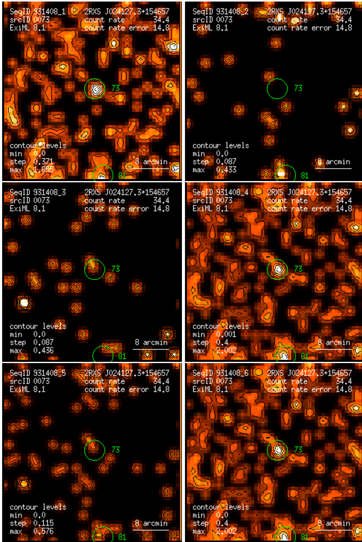
Figure 73: RASS 931408: detection 0073: band rate images, Gaussian filter: (1) PSPC channels 11 – 41, (2) 52 – 90, (3) 91 – 201, (4) 11 – 235, (5) 52 – 201, (6) 11 – 201. Broad band rates in counts/ks. Band rate contour levels in counts/ks/arcmin 2 .
