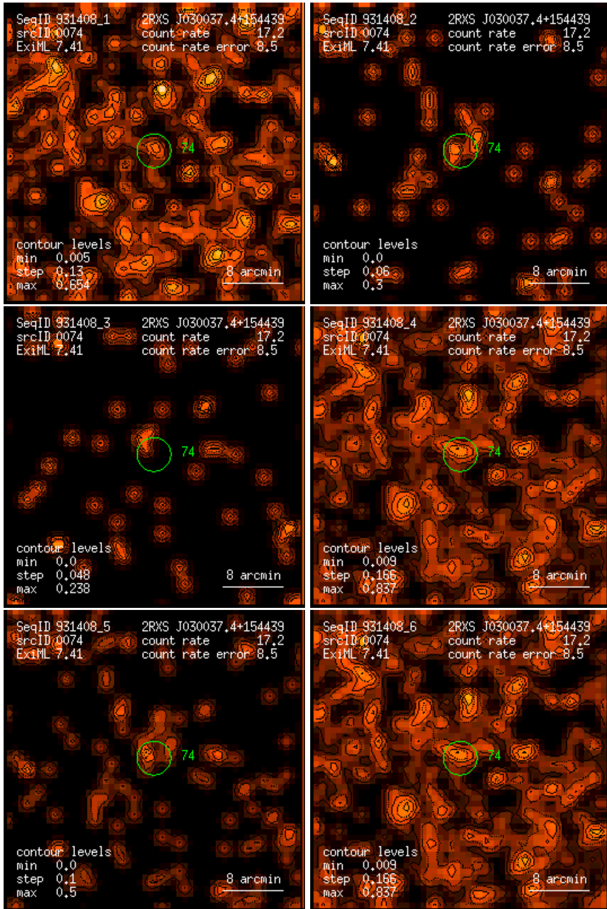
Figure 74: RASS 931408: detection 0074: band rate images, Gaussian filter: (1) PSPC channels 11 – 41, (2) 52 – 90, (3) 91 – 201, (4) 11 – 235, (5) 52 – 201, (6) 11 – 201. Broad band rates in counts/ks. Band rate contour levels in counts/ks/arcmin 2 .
