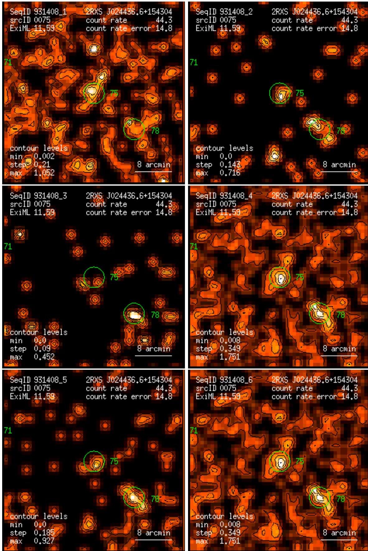
Figure 75: RASS 931408: detection 0075: band rate images, Gaussian filter: (1) PSPC channels 11 – 41, (2) 52 – 90, (3) 91 – 201, (4) 11 – 235, (5) 52 – 201, (6) 11 – 201. Broad band rates in counts/ks. Band rate contour levels in counts/ks/arcmin 2 .
