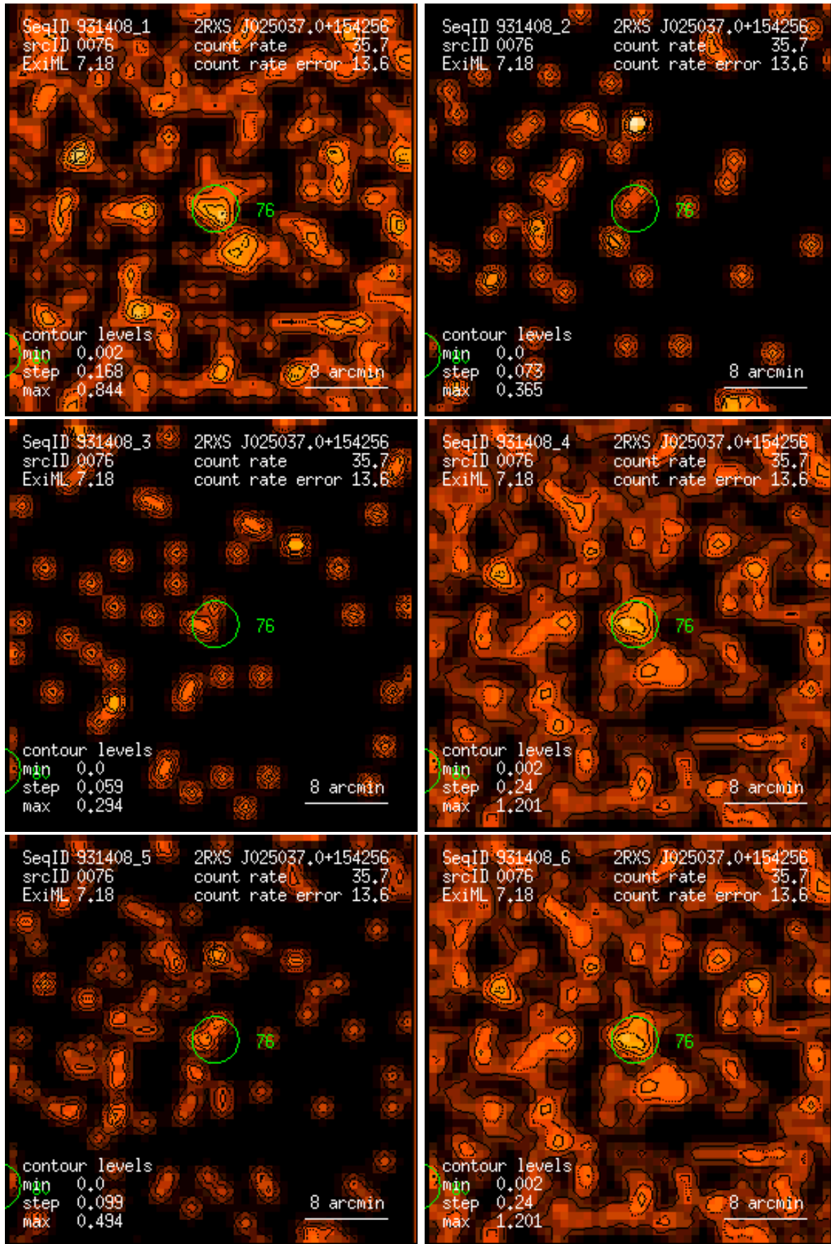
Figure 76: RASS 931408: detection 0076: band rate images, Gaussian filter: (1) PSPC channels 11 – 41, (2) 52 – 90, (3) 91 – 201, (4) 11 – 235, (5) 52 – 201, (6) 11 – 201. Broad band rates in counts/ks. Band rate contour levels in counts/ks/arcmin 2 .
