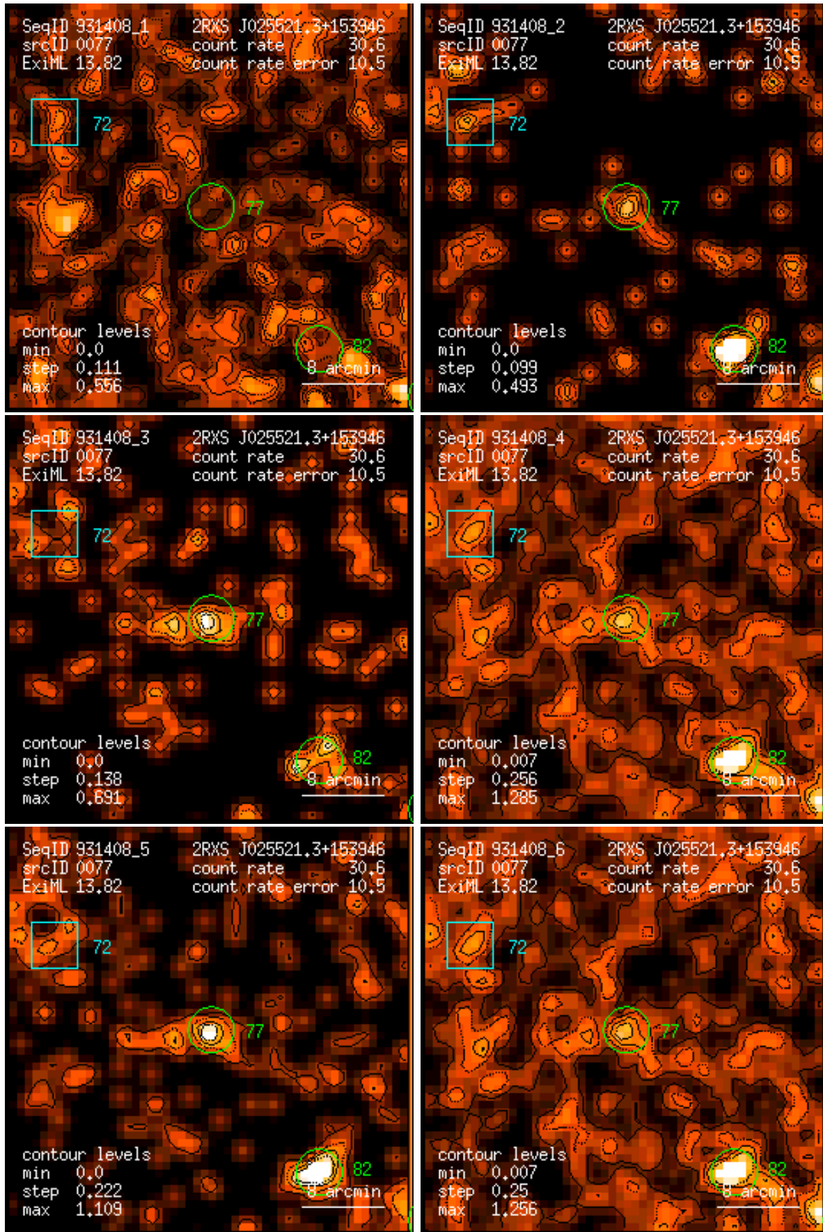
Figure 77: RASS 931408: detection 0077: band rate images, Gaussian filter: (1) PSPC channels 11 – 41, (2) 52 – 90, (3) 91 – 201, (4) 11 – 235, (5) 52 – 201, (6) 11 – 201. Broad band rates in counts/ks. Band rate contour levels in counts/ks/arcmin 2 .
