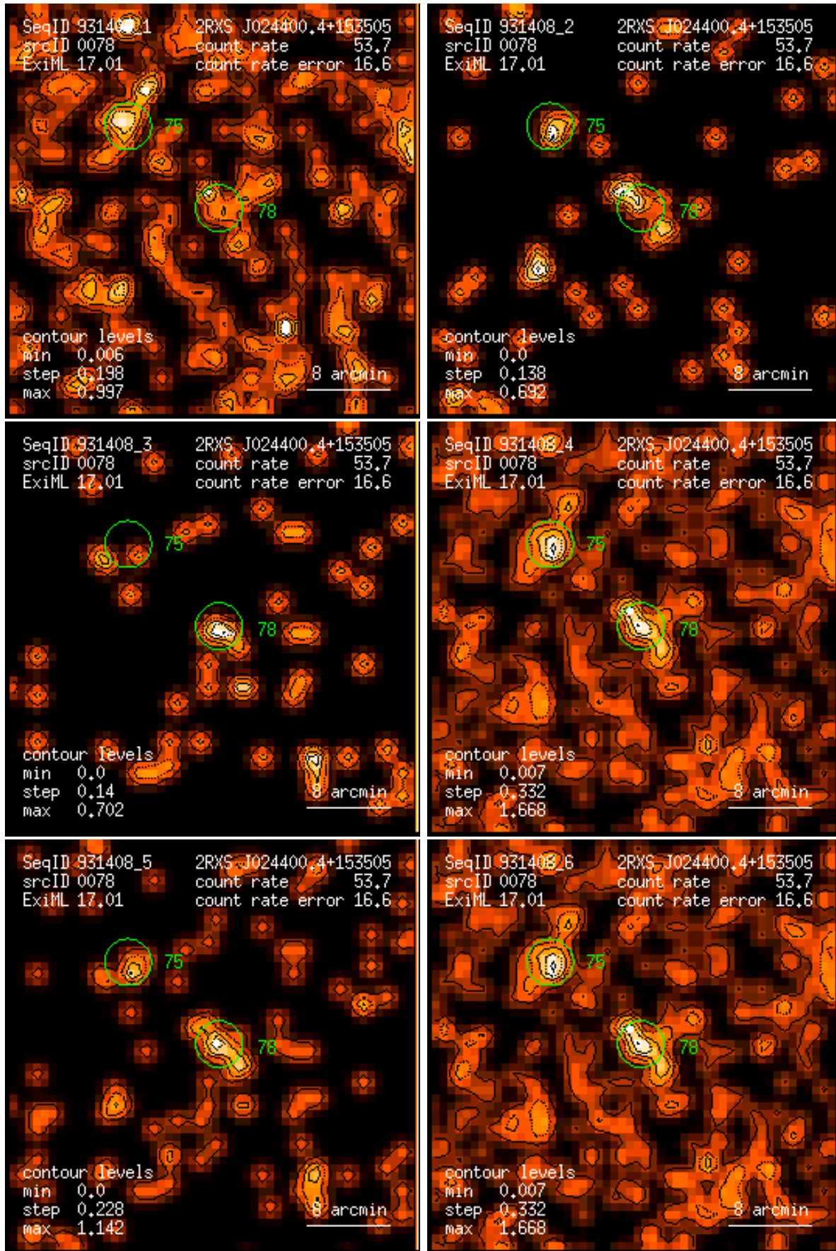
Figure 78: RASS 931408: detection 0078: band rate images, Gaussian filter: (1) PSPC channels 11 – 41, (2) 52 – 90, (3) 91 – 201, (4) 11 – 235, (5) 52 – 201, (6) 11 – 201. Broad band rates in counts/ks. Band rate contour levels in counts/ks/arcmin 2 .
