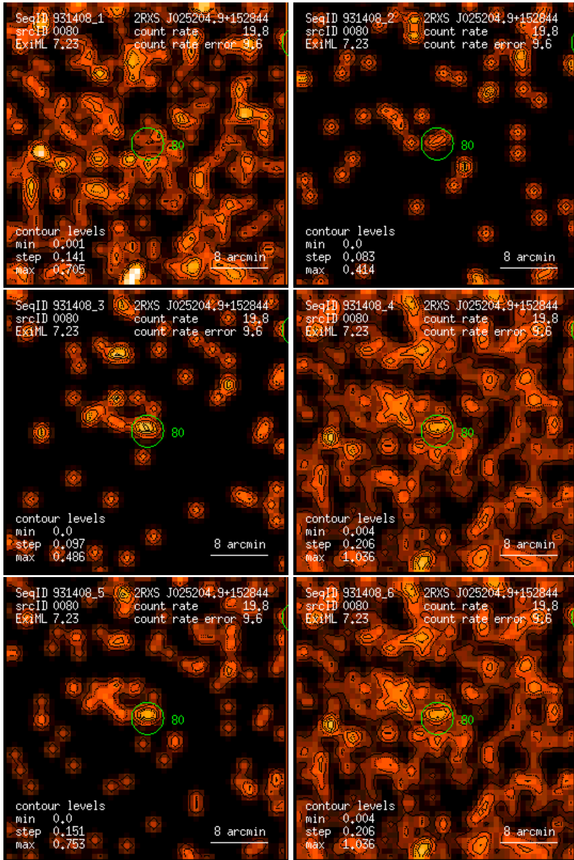
Figure 80: RASS 931408: detection 0080: band rate images, Gaussian filter: (1) PSPC channels 11 – 41, (2) 52 – 90, (3) 91 – 201, (4) 11 – 235, (5) 52 – 201, (6) 11 – 201. Broad band rates in counts/ks. Band rate contour levels in counts/ks/arcmin 2 .
