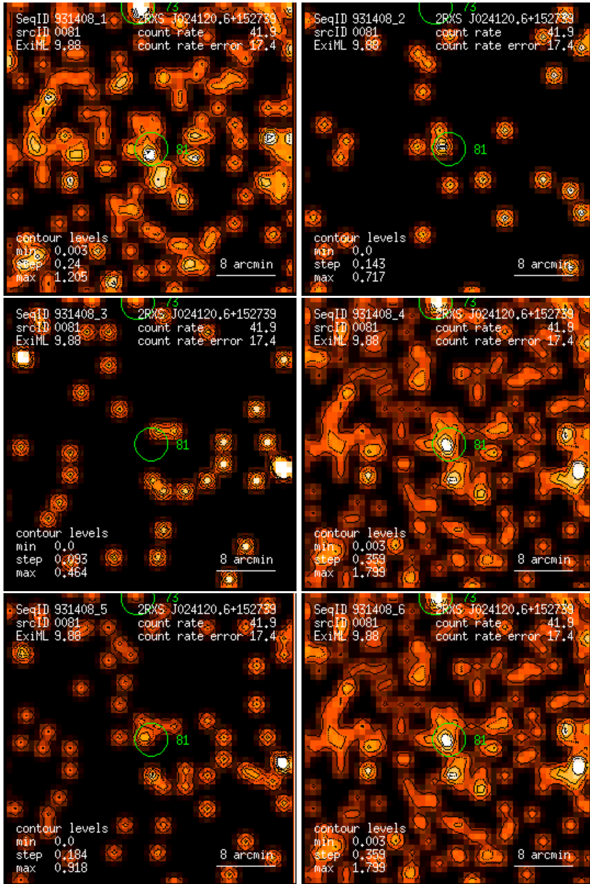
Figure 81: RASS 931408: detection 0081: band rate images, Gaussian filter: (1) PSPC channels 11 – 41, (2) 52 – 90, (3) 91 – 201, (4) 11 – 235, (5) 52 – 201, (6) 11 – 201. Broad band rates in counts/ks. Band rate contour levels in counts/ks/arcmin 2 .
