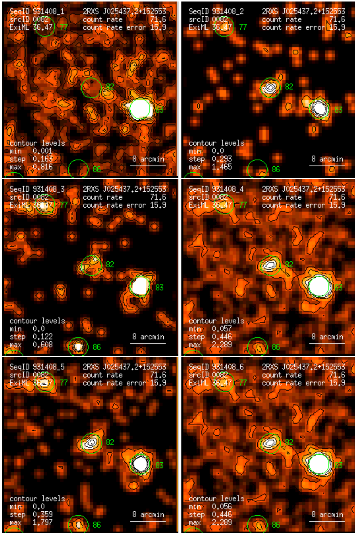
Figure 82: RASS 931408: detection 0082: band rate images, Gaussian filter: (1) PSPC channels 11 – 41, (2) 52 – 90, (3) 91 – 201, (4) 11 – 235, (5) 52 – 201, (6) 11 – 201. Broad band rates in counts/ks. Band rate contour levels in counts/ks/arcmin 2 .
