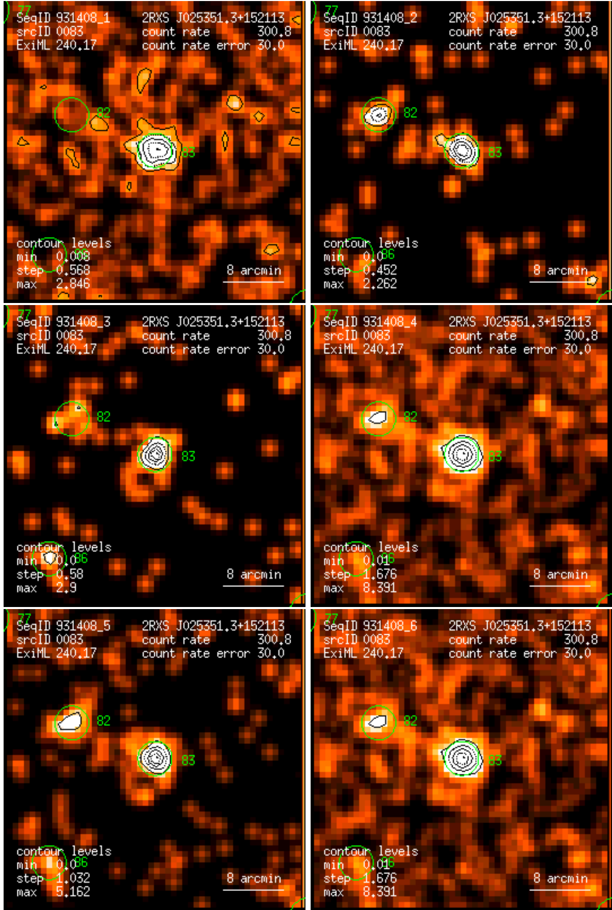
Figure 83: RASS 931408: detection 0083: band rate images, Gaussian filter: (1) PSPC channels 11 – 41, (2) 52 – 90, (3) 91 – 201, (4) 11 – 235, (5) 52 – 201, (6) 11 – 201. Broad band rates in counts/ks. Band rate contour levels in counts/ks/arcmin 2 .
