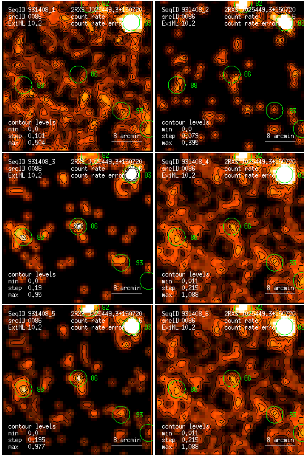
Figure 86: RASS 931408: detection 0086: band rate images, Gaussian filter: (1) PSPC channels 11 – 41, (2) 52 – 90, (3) 91 – 201, (4) 11 – 235, (5) 52 – 201, (6) 11 – 201. Broad band rates in counts/ks. Band rate contour levels in counts/ks/arcmin 2 .
