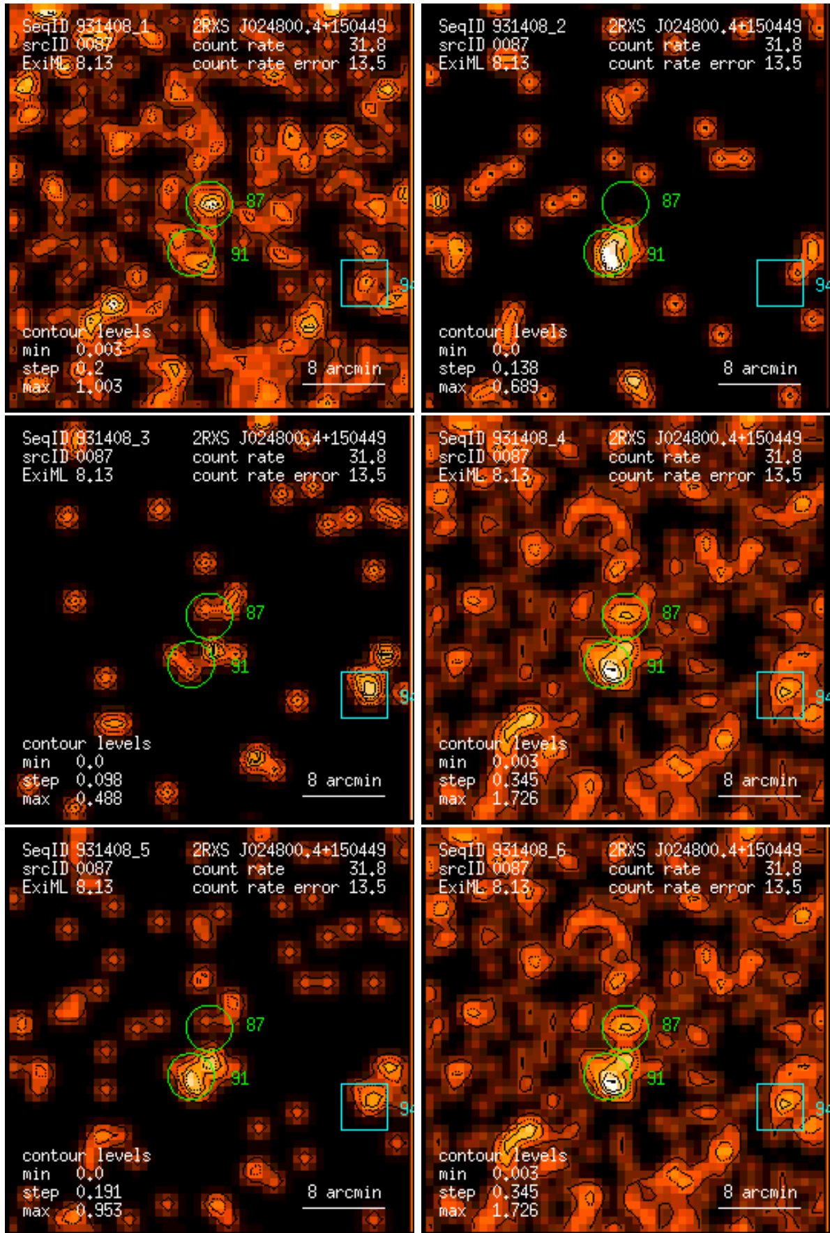
Figure 87: RASS 931408: detection 0087: band rate images, Gaussian filter: (1) PSPC channels 11 – 41, (2) 52 – 90, (3) 91 – 201, (4) 11 – 235, (5) 52 – 201, (6) 11 – 201. Broad band rates in counts/ks. Band rate contour levels in counts/ks/arcmin 2 .
