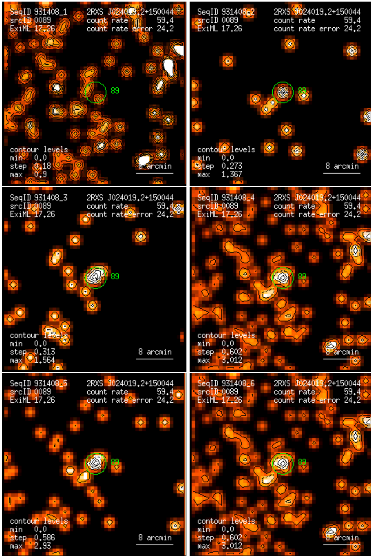
Figure 89: RASS 931408: detection 0089: band rate images, Gaussian filter: (1) PSPC channels 11 – 41, (2) 52 – 90, (3) 91 – 201, (4) 11 – 235, (5) 52 – 201, (6) 11 – 201. Broad band rates in counts/ks. Band rate contour levels in counts/ks/arcmin 2 .
