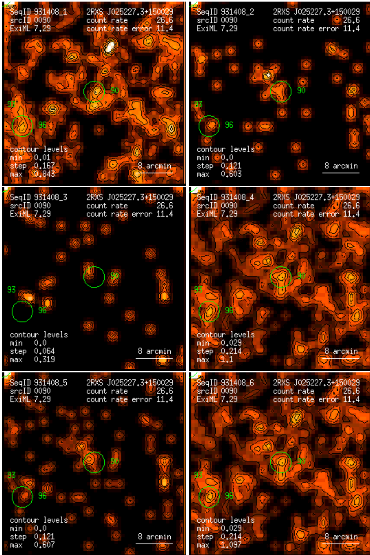
Figure 90: RASS 931408: detection 0090: band rate images, Gaussian filter: (1) PSPC channels 11 – 41, (2) 52 – 90, (3) 91 – 201, (4) 11 – 235, (5) 52 – 201, (6) 11 – 201. Broad band rates in counts/ks. Band rate contour levels in counts/ks/arcmin 2 .
