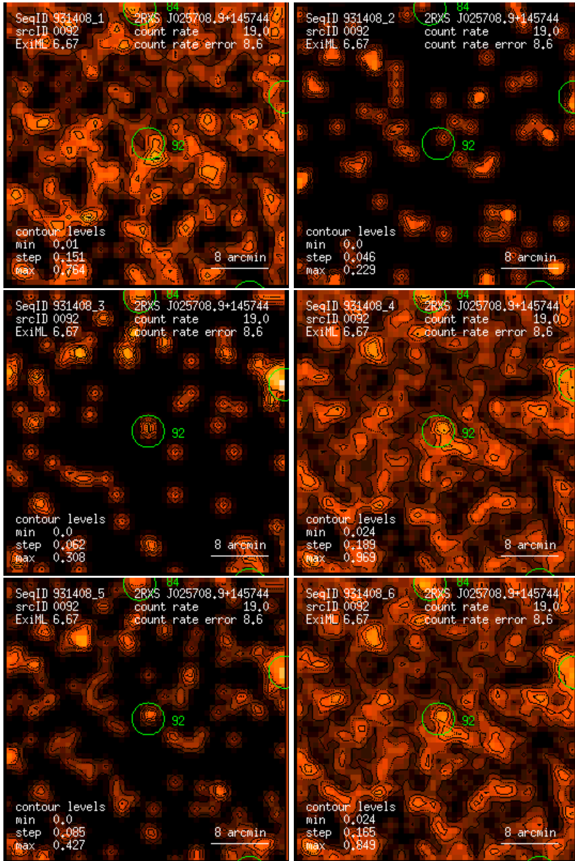
Figure 92: RASS 931408: detection 0092: band rate images, Gaussian filter: (1) PSPC channels 11 – 41, (2) 52 – 90, (3) 91 – 201, (4) 11 – 235, (5) 52 – 201, (6) 11 – 201. Broad band rates in counts/ks. Band rate contour levels in counts/ks/arcmin 2 .
