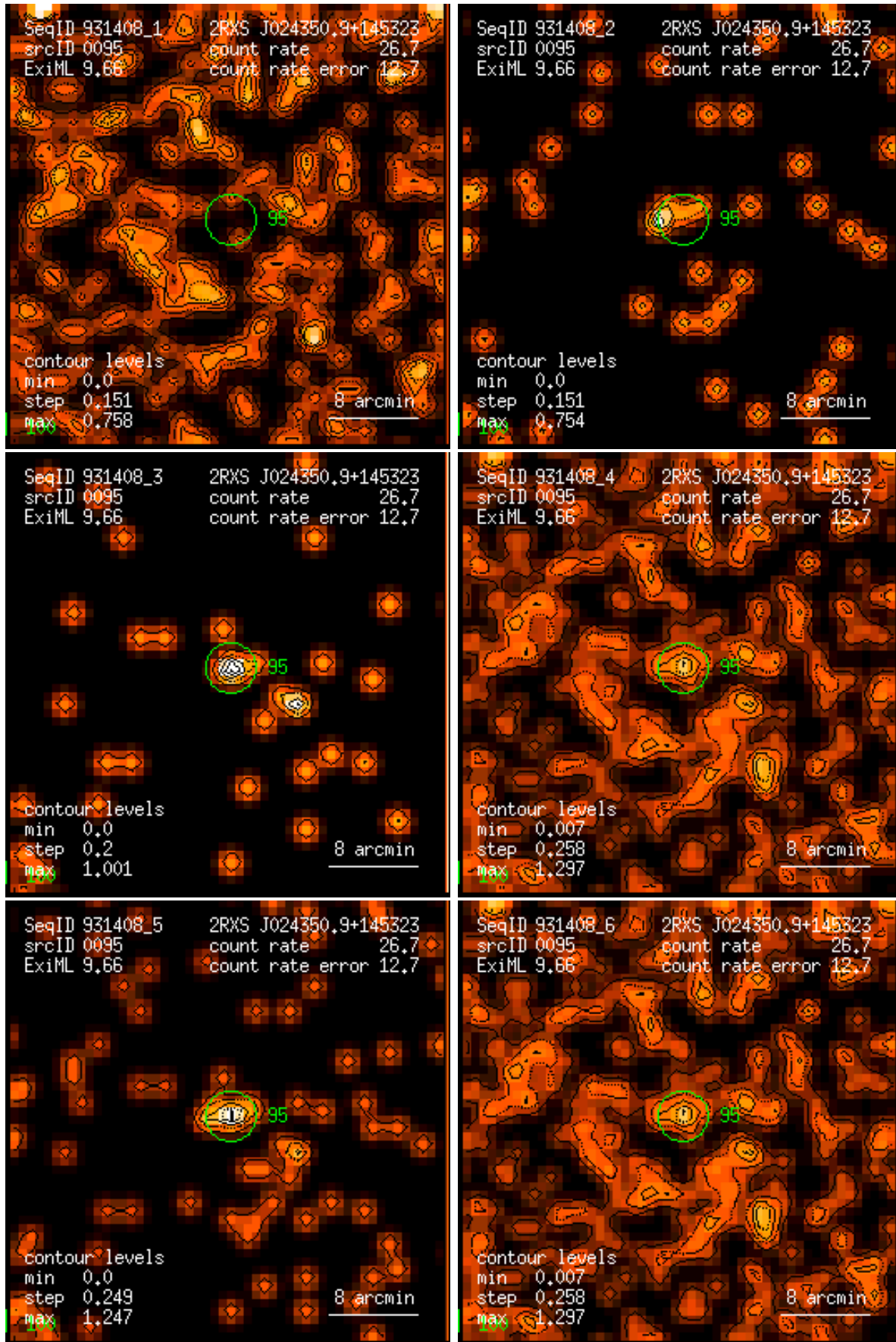
Figure 95: RASS 931408: detection 0095: band rate images, Gaussian filter: (1) PSPC channels 11 – 41, (2) 52 – 90, (3) 91 – 201, (4) 11 – 235, (5) 52 – 201, (6) 11 – 201. Broad band rates in counts/ks. Band rate contour levels in counts/ks/arcmin 2 .
