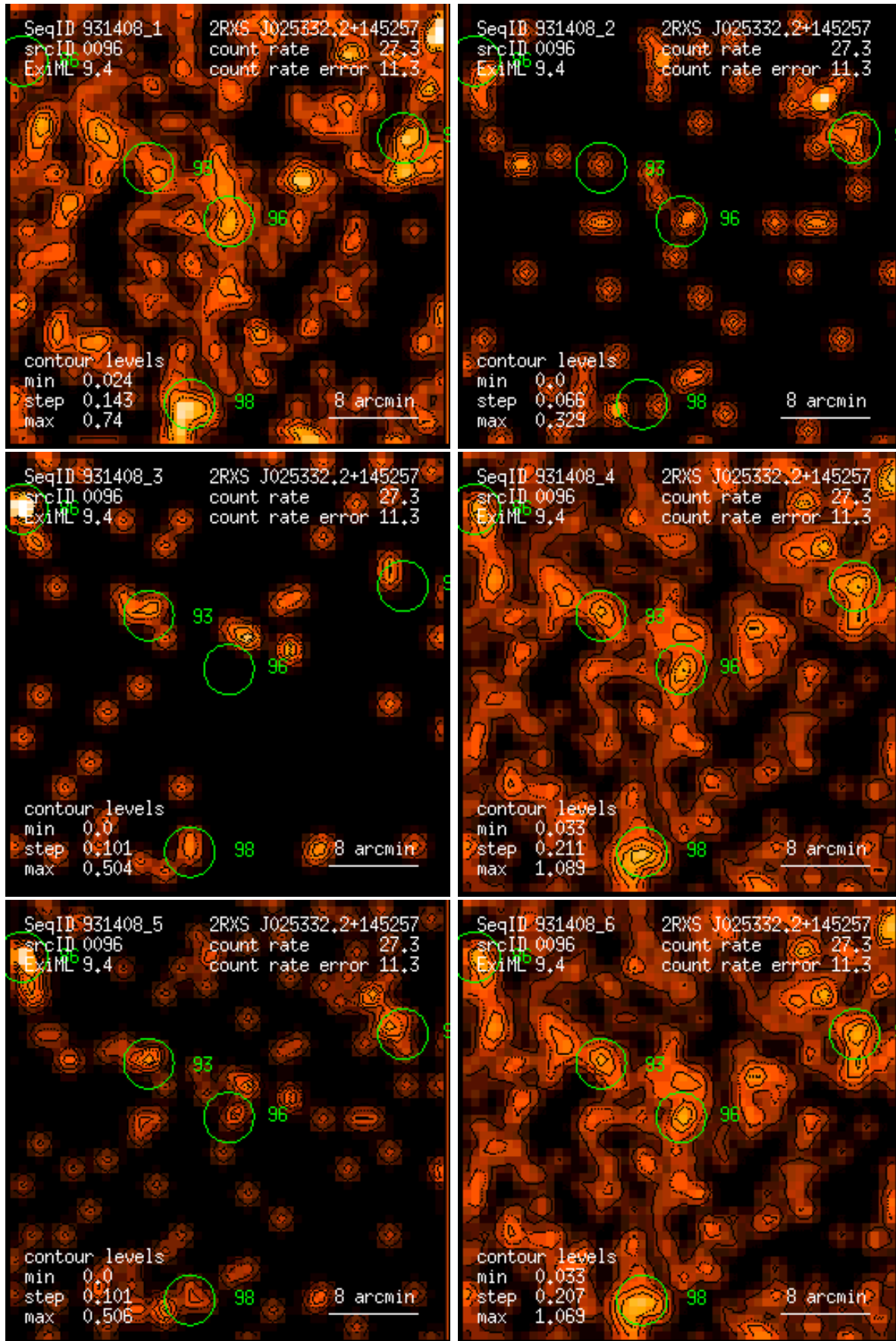
Figure 96: RASS 931408: detection 0096: band rate images, Gaussian filter: (1) PSPC channels 11 – 41, (2) 52 – 90, (3) 91 – 201, (4) 11 – 235, (5) 52 – 201, (6) 11 – 201. Broad band rates in counts/ks. Band rate contour levels in counts/ks/arcmin 2 .
