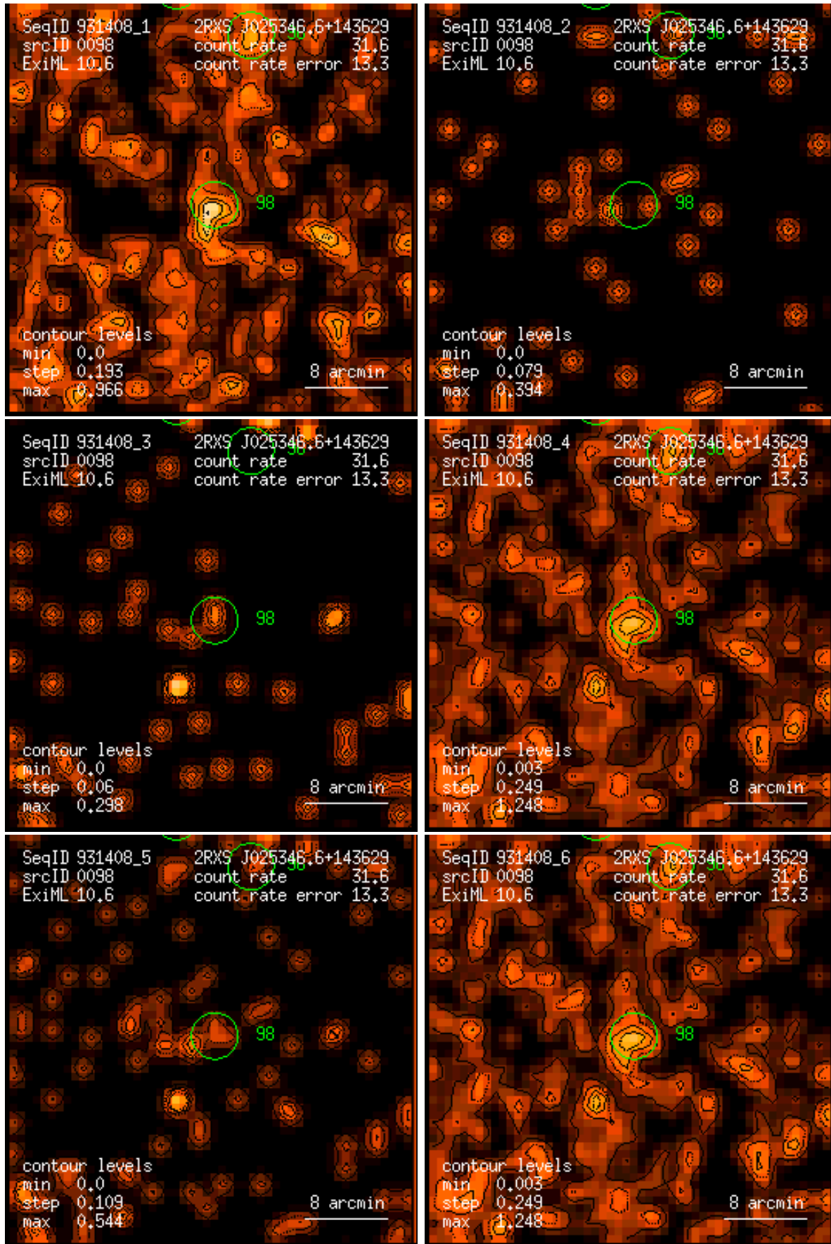
Figure 98: RASS 931408: detection 0098: band rate images, Gaussian filter: (1) PSPC channels 11 – 41, (2) 52 – 90, (3) 91 – 201, (4) 11 – 235, (5) 52 – 201, (6) 11 – 201. Broad band rates in counts/ks. Band rate contour levels in counts/ks/arcmin 2 .
