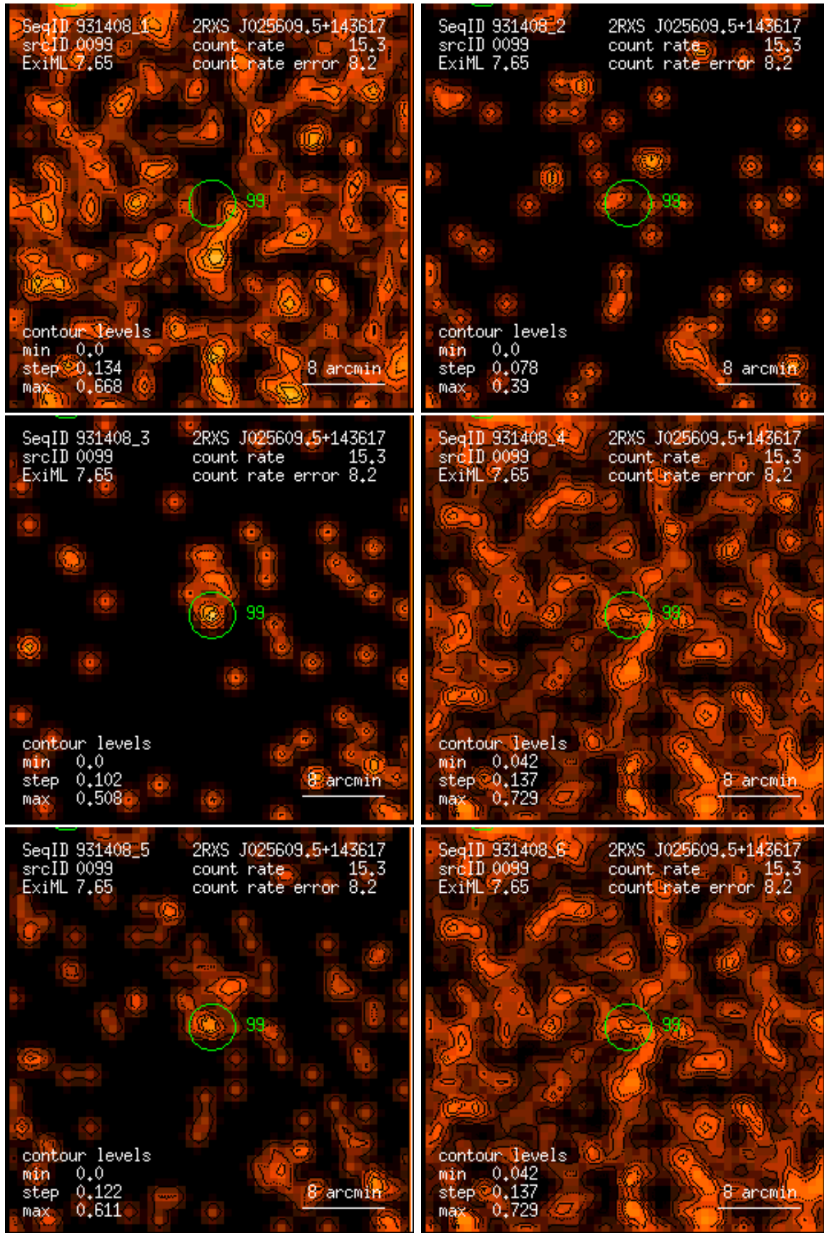
Figure 99: RASS 931408: detection 0099: band rate images, Gaussian filter: (1) PSPC channels 11 – 41, (2) 52 – 90, (3) 91 – 201, (4) 11 – 235, (5) 52 – 201, (6) 11 – 201. Broad band rates in counts/ks. Band rate contour levels in counts/ks/arcmin 2 .
