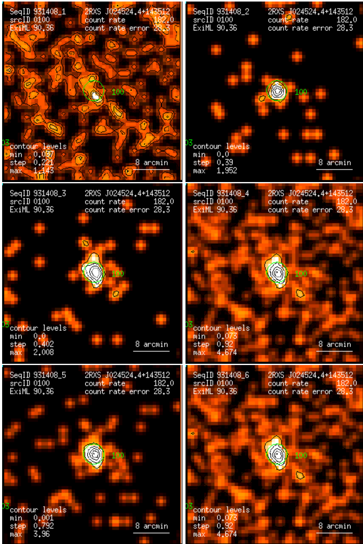
Figure 100: RASS 931408: detection 0100: band rate images, Gaussian filter: (1) PSPC channels 11 – 41, (2) 52 – 90, (3) 91 – 201, (4) 11 – 235, (5) 52 – 201, (6) 11 – 201. Broad band rates in counts/ks. Band rate contour levels in counts/ks/arcmin 2 .
