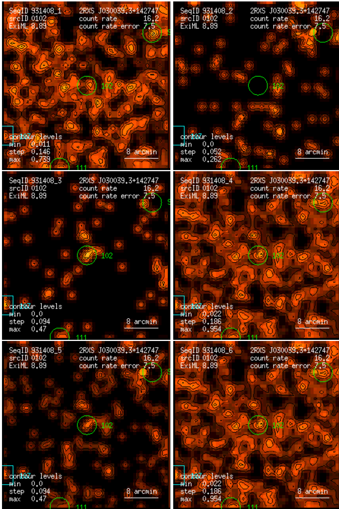
Figure 102: RASS 931408: detection 0102: band rate images, Gaussian filter: (1) PSPC channels 11 – 41, (2) 52 – 90, (3) 91 – 201, (4) 11 – 235, (5) 52 – 201, (6) 11 – 201. Broad band rates in counts/ks. Band rate contour levels in counts/ks/arcmin 2 .
