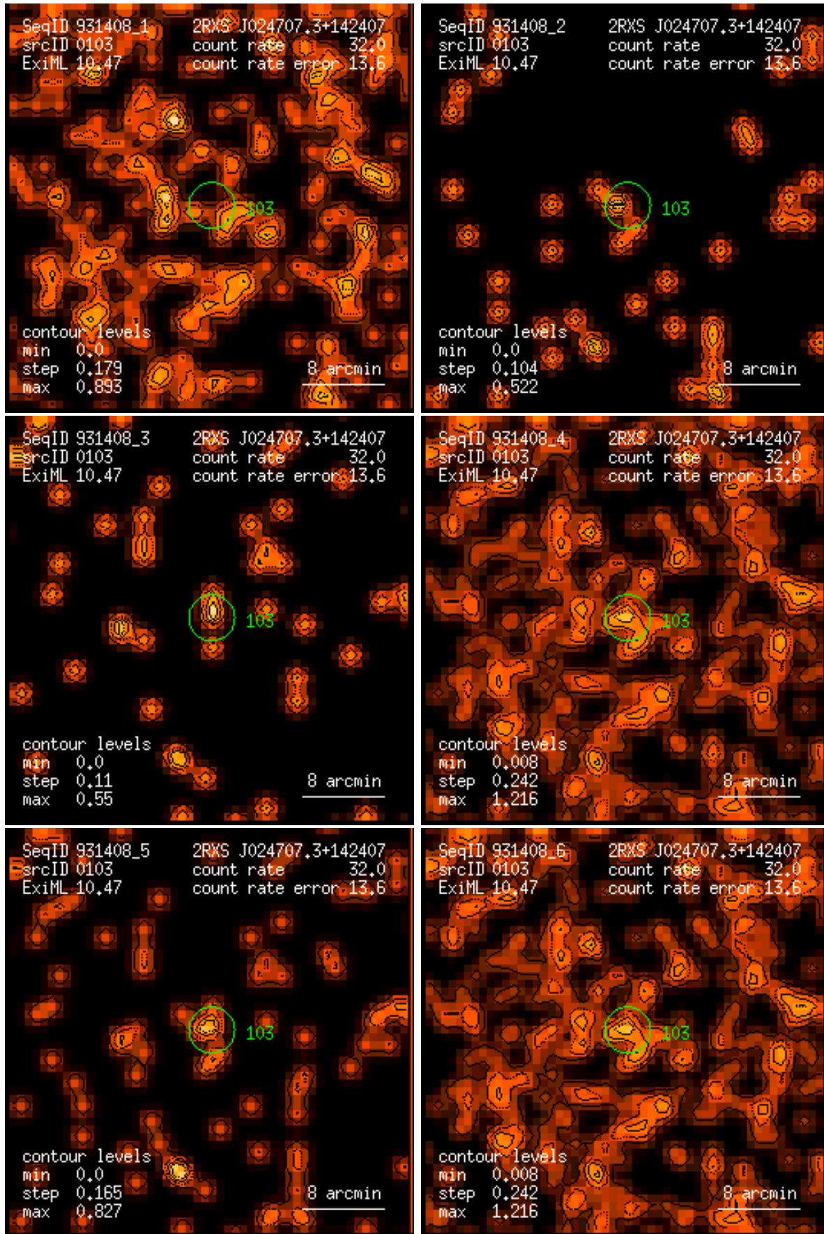
Figure 103: RASS 931408: detection 0103: band rate images, Gaussian filter: (1) PSPC channels 11 – 41, (2) 52 – 90, (3) 91 – 201, (4) 11 – 235, (5) 52 – 201, (6) 11 – 201. Broad band rates in counts/ks. Band rate contour levels in counts/ks/arcmin 2 .
