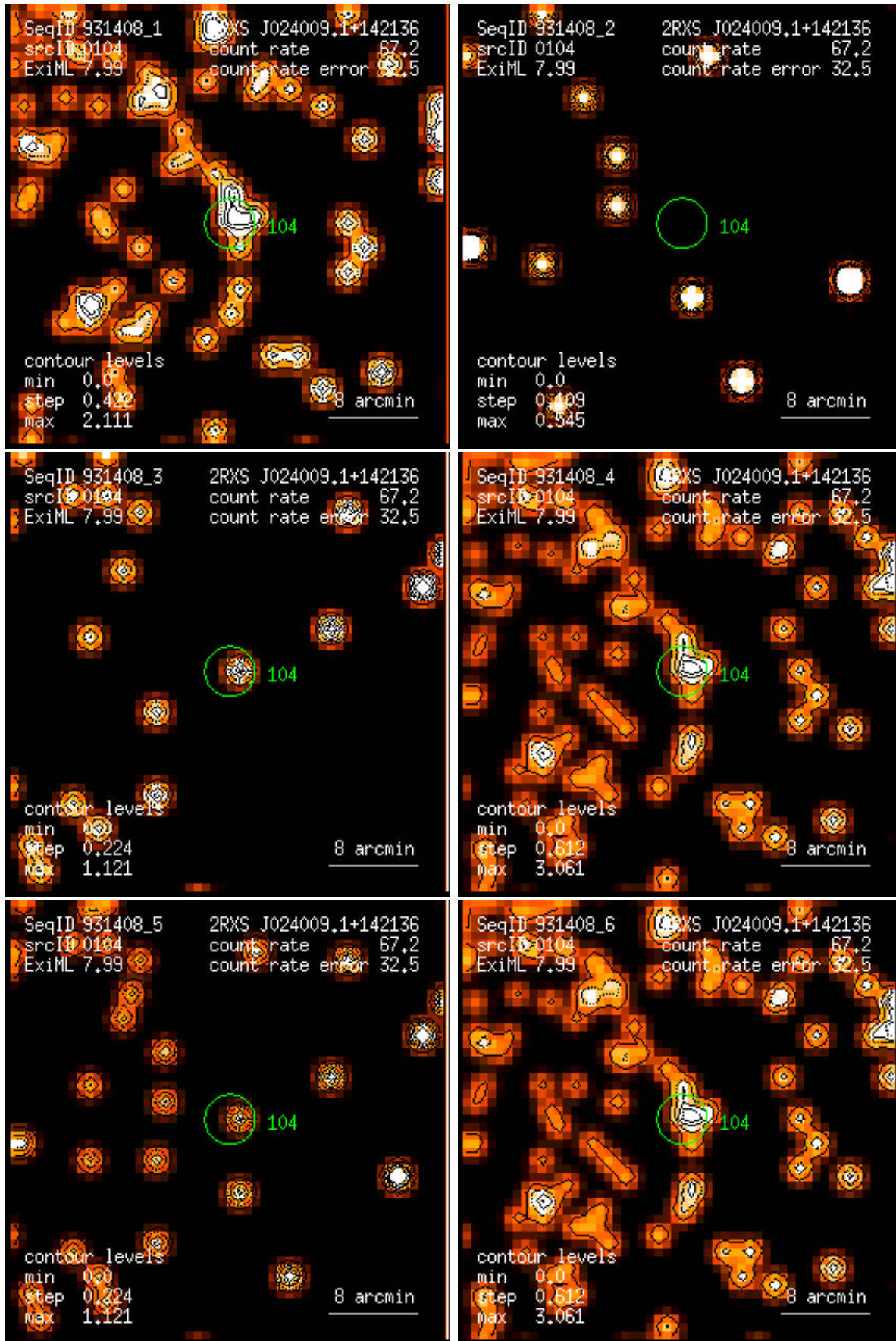
Figure 104: RASS 931408: detection 0104: band rate images, Gaussian filter: (1) PSPC channels 11 – 41, (2) 52 – 90, (3) 91 – 201, (4) 11 – 235, (5) 52 – 201, (6) 11 – 201. Broad band rates in counts/ks. Band rate contour levels in counts/ks/arcmin 2 .
