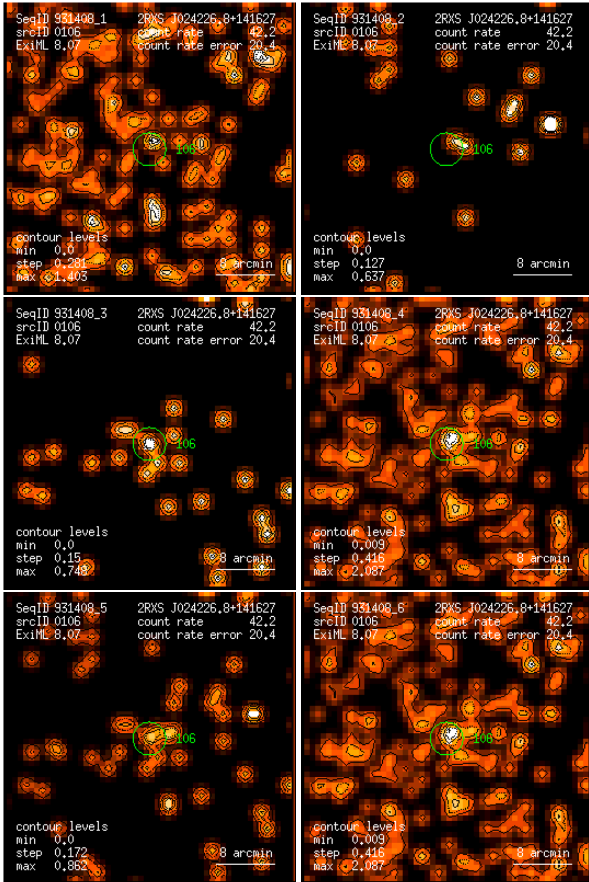
Figure 106: RASS 931408: detection 0106: band rate images, Gaussian filter: (1) PSPC channels 11 – 41, (2) 52 – 90, (3) 91 – 201, (4) 11 – 235, (5) 52 – 201, (6) 11 – 201. Broad band rates in counts/ks. Band rate contour levels in counts/ks/arcmin 2 .
