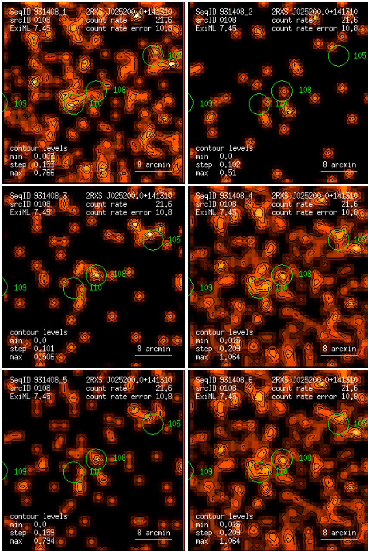
Figure 108: RASS 931408: detection 0108: band rate images, Gaussian filter: (1) PSPC channels 11 – 41, (2) 52 – 90, (3) 91 – 201, (4) 11 – 235, (5) 52 – 201, (6) 11 – 201. Broad band rates in counts/ks. Band rate contour levels in counts/ks/arcmin 2 .
