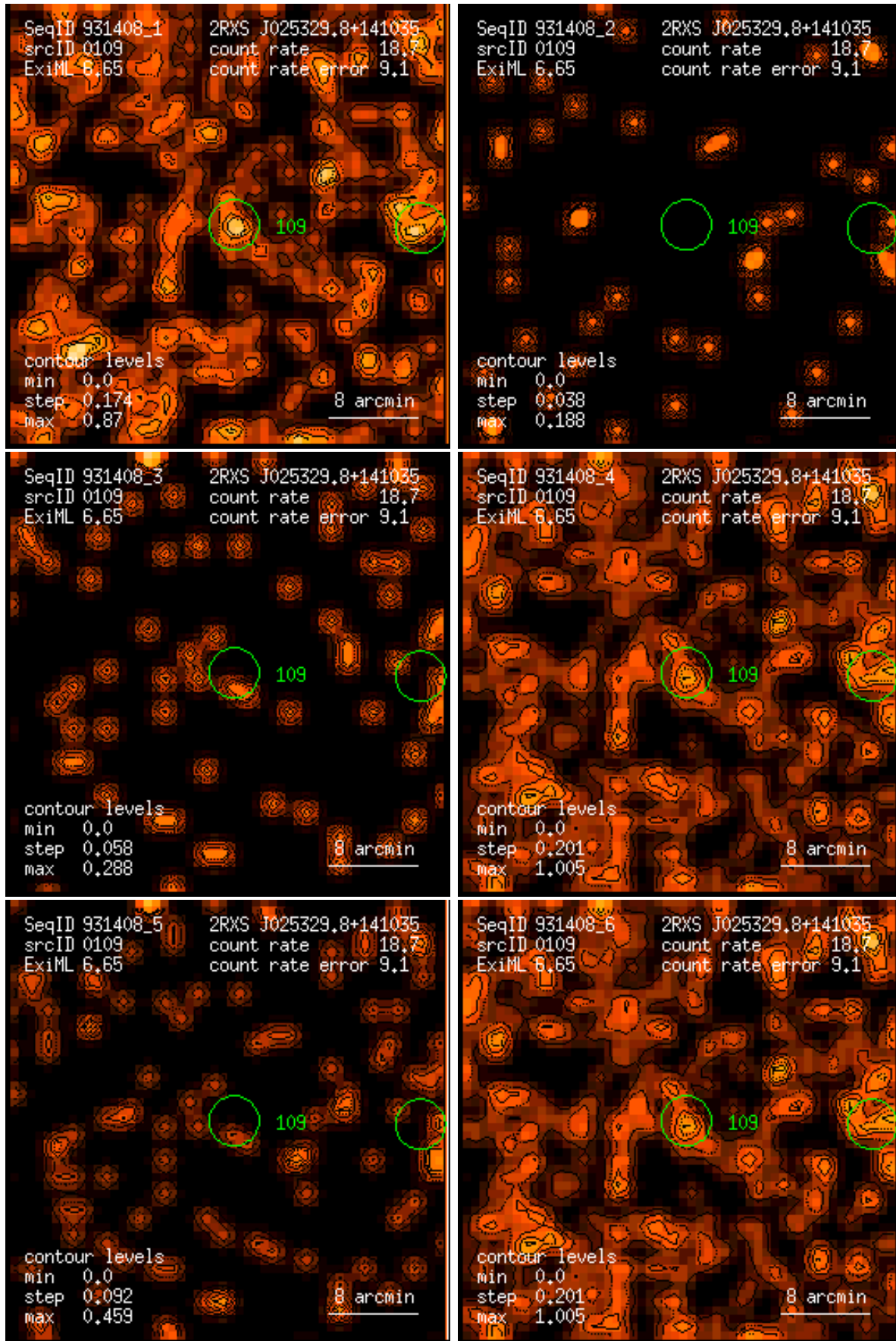
Figure 109: RASS 931408: detection 0109: band rate images, Gaussian filter: (1) PSPC channels 11 – 41, (2) 52 – 90, (3) 91 – 201, (4) 11 – 235, (5) 52 – 201, (6) 11 – 201. Broad band rates in counts/ks. Band rate contour levels in counts/ks/arcmin 2 .
