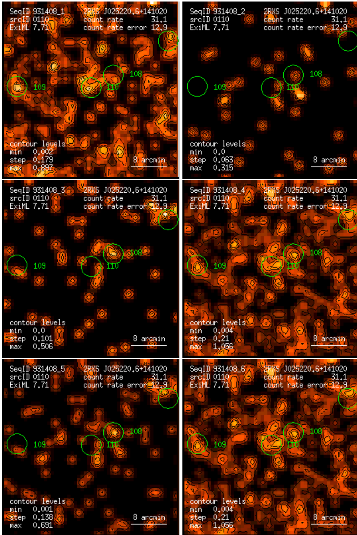
Figure 110: RASS 931408: detection 0110: band rate images, Gaussian filter: (1) PSPC channels 11 – 41, (2) 52 – 90, (3) 91 – 201, (4) 11 – 235, (5) 52 – 201, (6) 11 – 201. Broad band rates in counts/ks. Band rate contour levels in counts/ks/arcmin 2 .
