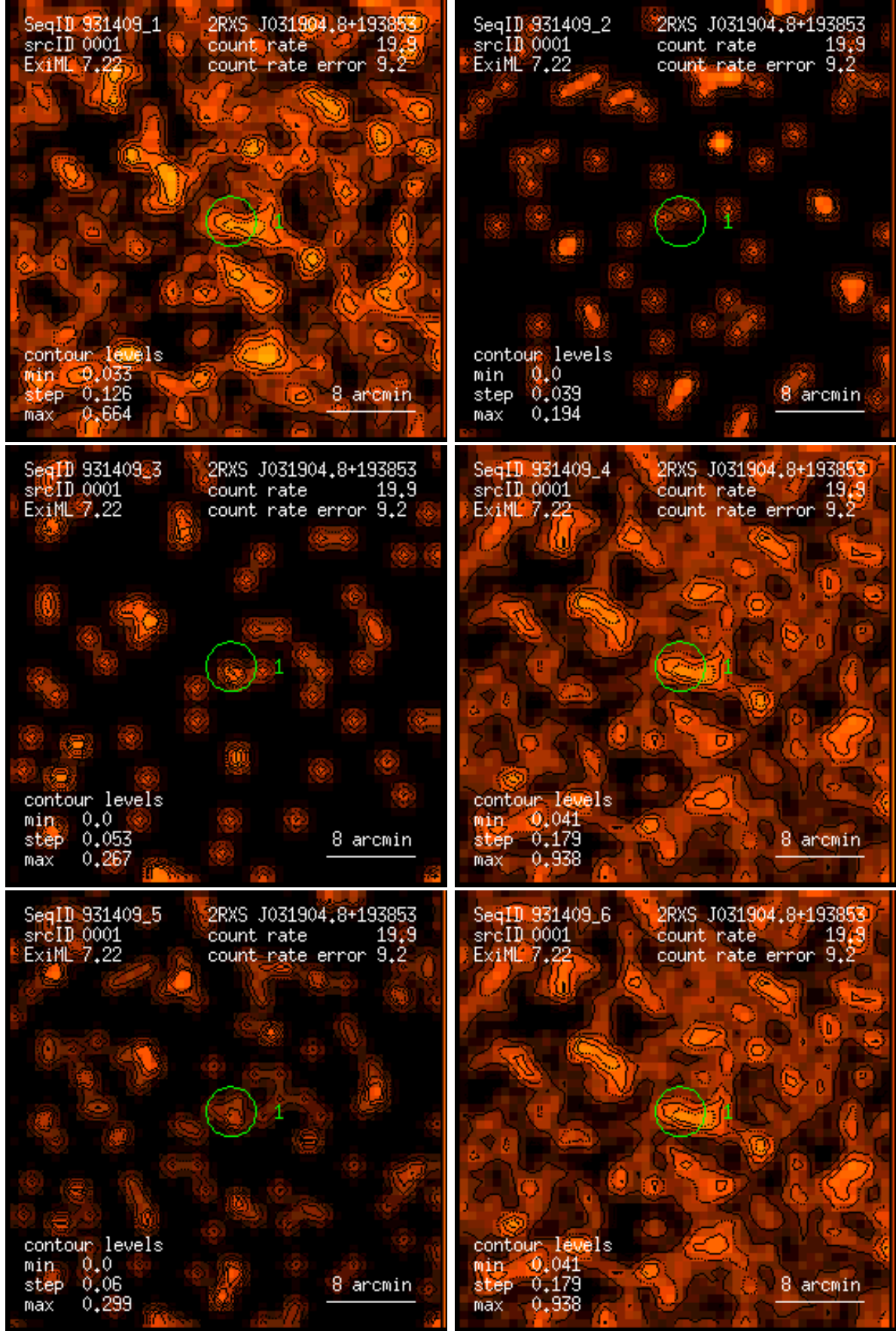
Figure 1: RASS 931409: detection 0001: band rate images, Gaussian filter: (1) PSPC channels 11 – 41, (2) 52 – 90, (3) 91 – 201, (4) 11 – 235, (5) 52 – 201, (6) 11 – 201. Broad band rates in counts/ks. Band rate contour levels in counts/ks/arcmin 2 .
