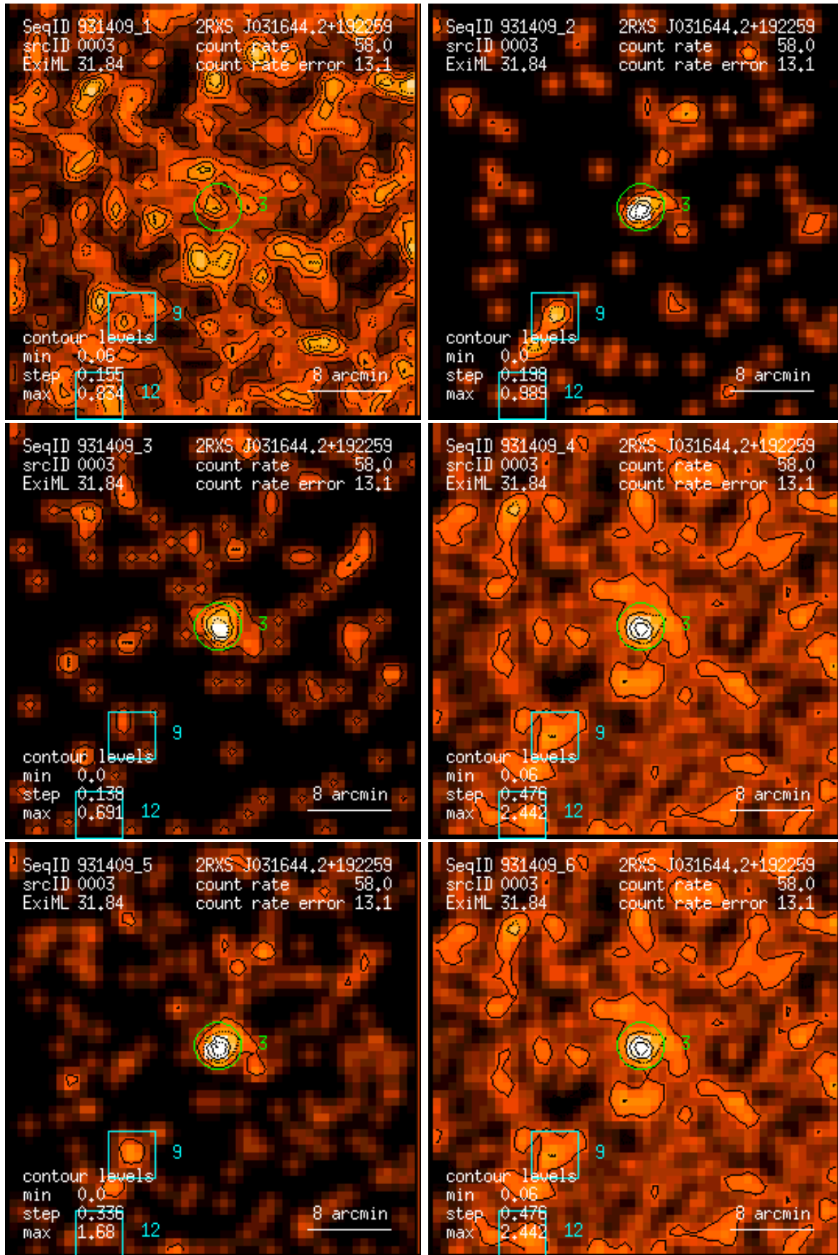
Figure 3: RASS 931409: detection 0003: band rate images, Gaussian filter: (1) PSPC channels 11 – 41, (2) 52 – 90, (3) 91 – 201, (4) 11 – 235, (5) 52 – 201, (6) 11 – 201. Broad band rates in counts/ks. Band rate contour levels in counts/ks/arcmin 2 .
