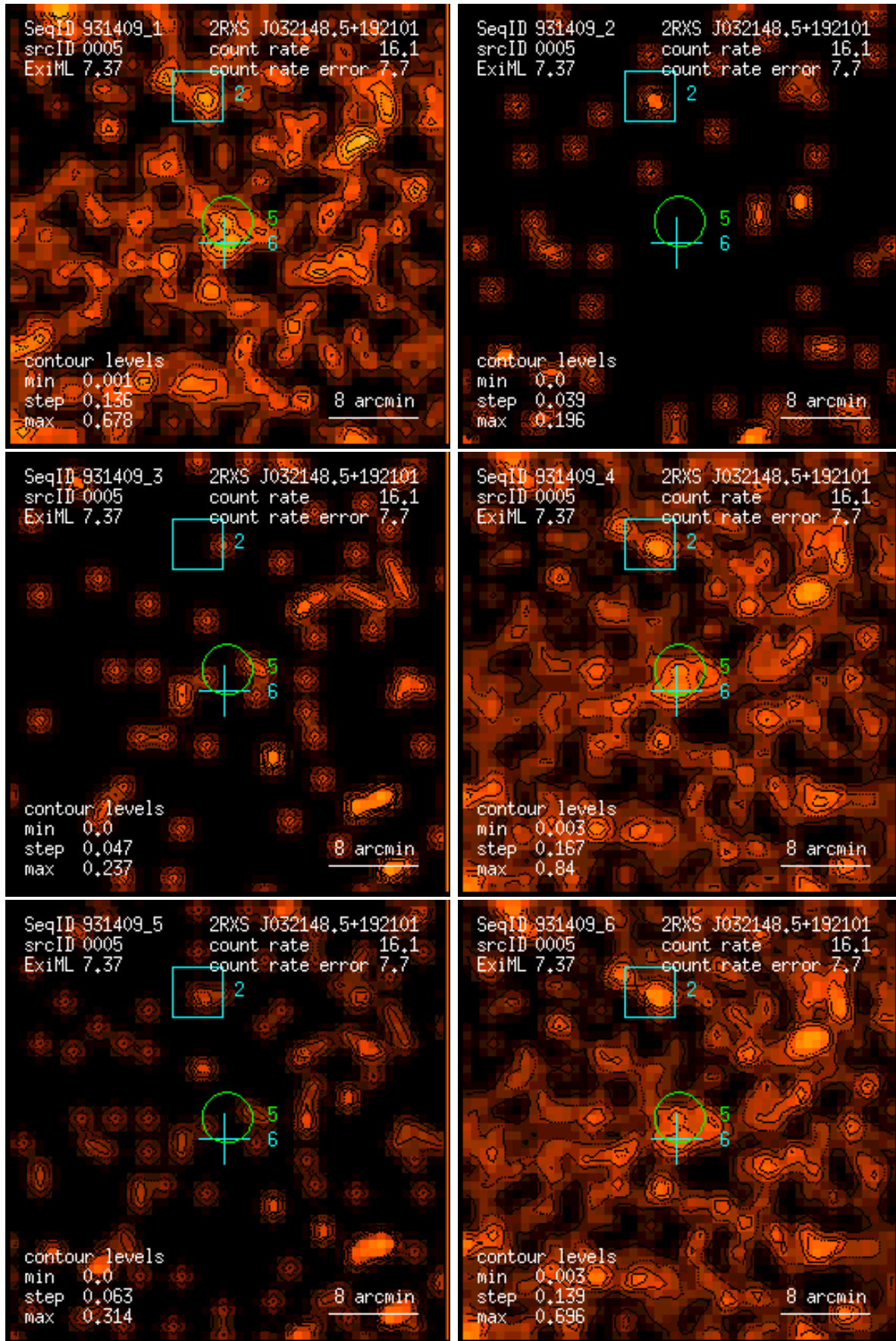
Figure 5: RASS 931409: detection 0005: band rate images, Gaussian filter: (1) PSPC channels 11 – 41, (2) 52 – 90, (3) 91 – 201, (4) 11 – 235, (5) 52 – 201, (6) 11 – 201. Broad band rates in counts/ks. Band rate contour levels in counts/ks/arcmin 2 .
