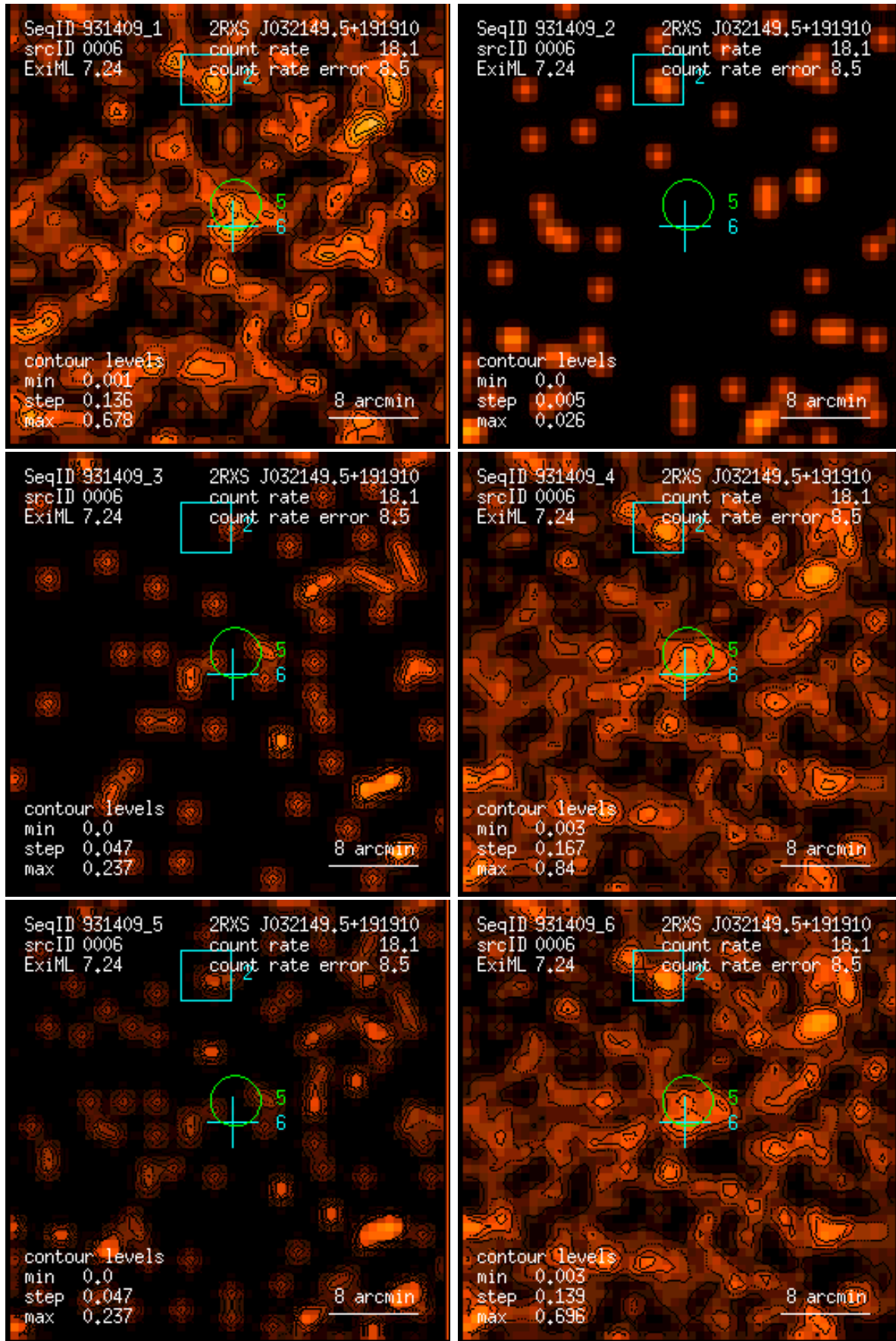
Figure 6: RASS 931409: detection 0006: band rate images, Gaussian filter: (1) PSPC channels 11 – 41, (2) 52 – 90, (3) 91 – 201, (4) 11 – 235, (5) 52 – 201, (6) 11 – 201. Broad band rates in counts/ks. Band rate contour levels in counts/ks/arcmin 2 .
