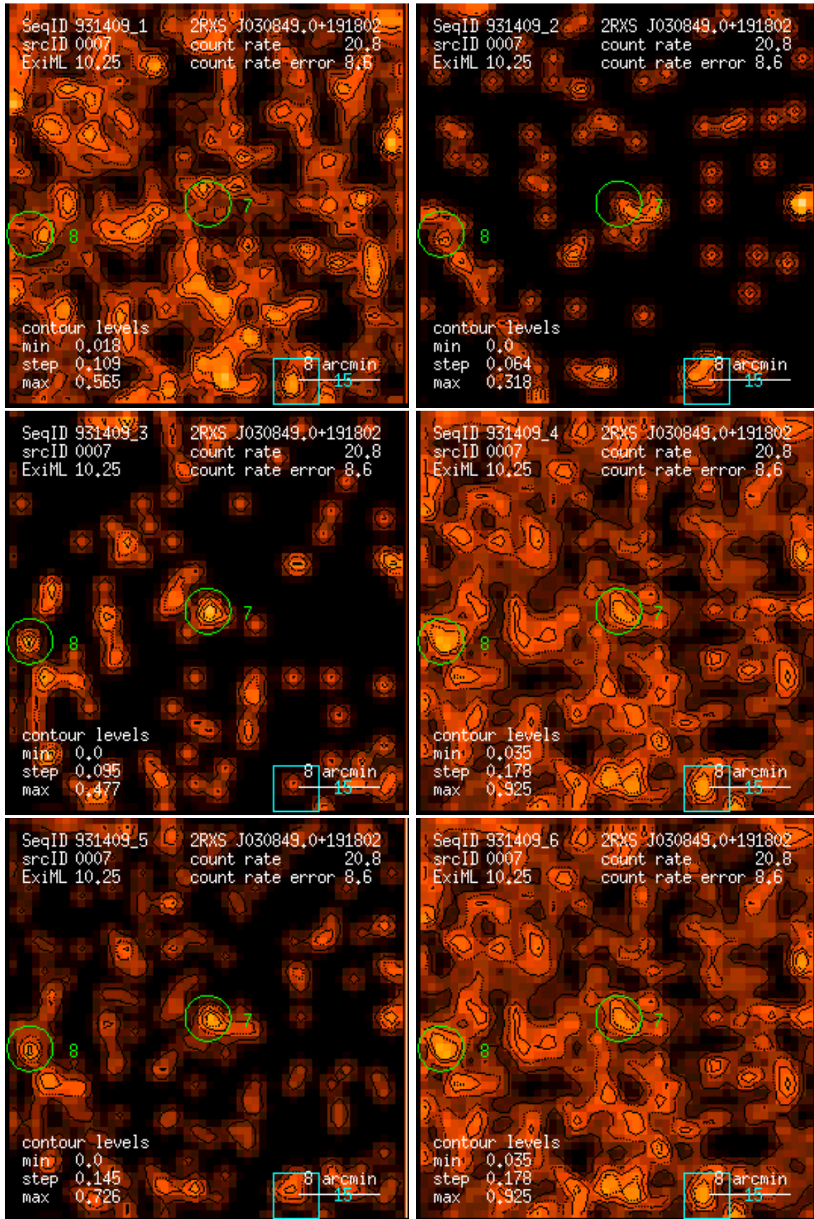
Figure 7: RASS 931409: detection 0007: band rate images, Gaussian filter: (1) PSPC channels 11 – 41, (2) 52 – 90, (3) 91 – 201, (4) 11 – 235, (5) 52 – 201, (6) 11 – 201. Broad band rates in counts/ks. Band rate contour levels in counts/ks/arcmin 2 .
