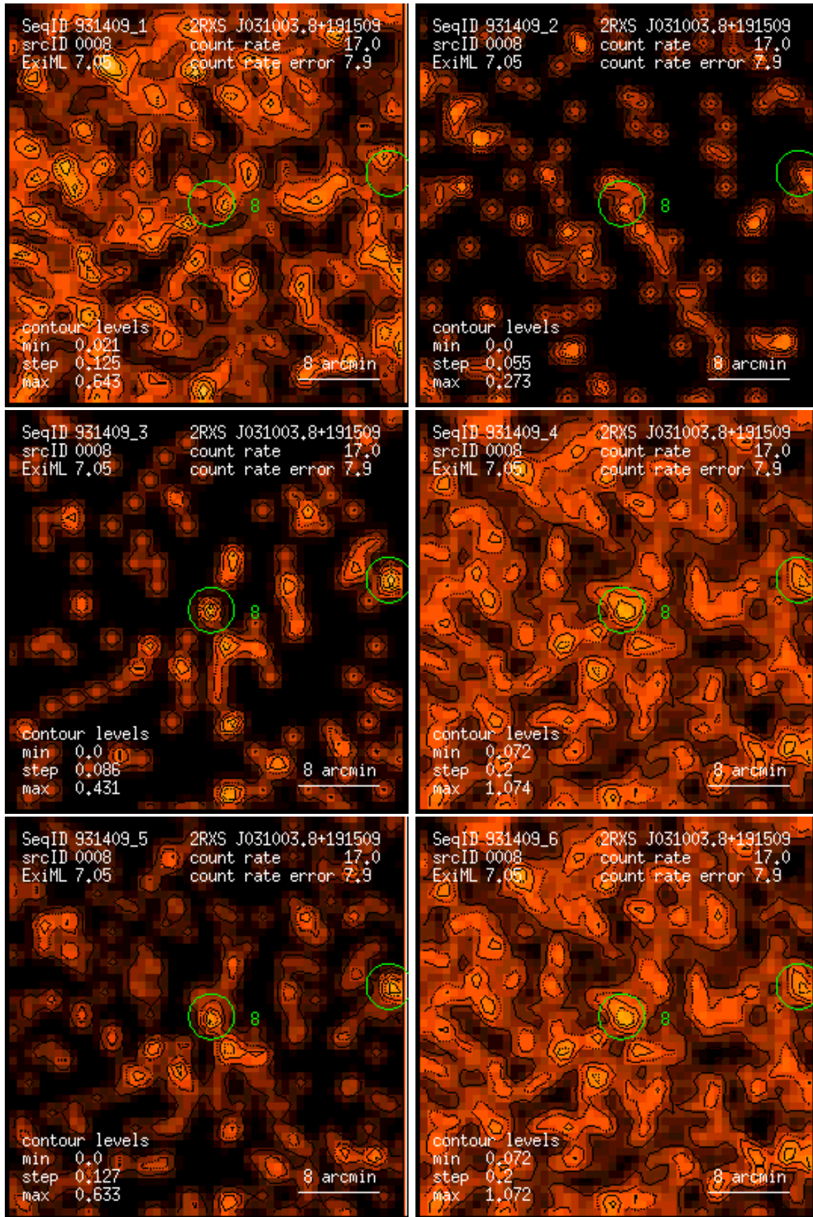
Figure 8: RASS 931409: detection 0008: band rate images, Gaussian filter: (1) PSPC channels 11 – 41, (2) 52 – 90, (3) 91 – 201, (4) 11 – 235, (5) 52 – 201, (6) 11 – 201. Broad band rates in counts/ks. Band rate contour levels in counts/ks/arcmin 2 .
